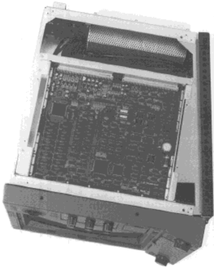
PHOTO 4 RIGHT SIDE VIEW OF DISPLAY UNIT NCD-3780
