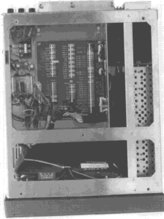
PHOTO 6 TOP VIEW OF DISPLAY UNIT NCD-5760
