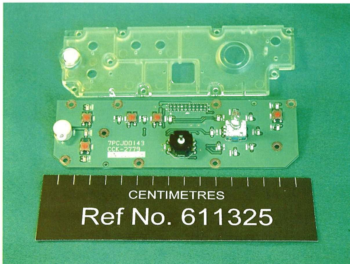
NCM-779 AIS Controller – Internal View 3
