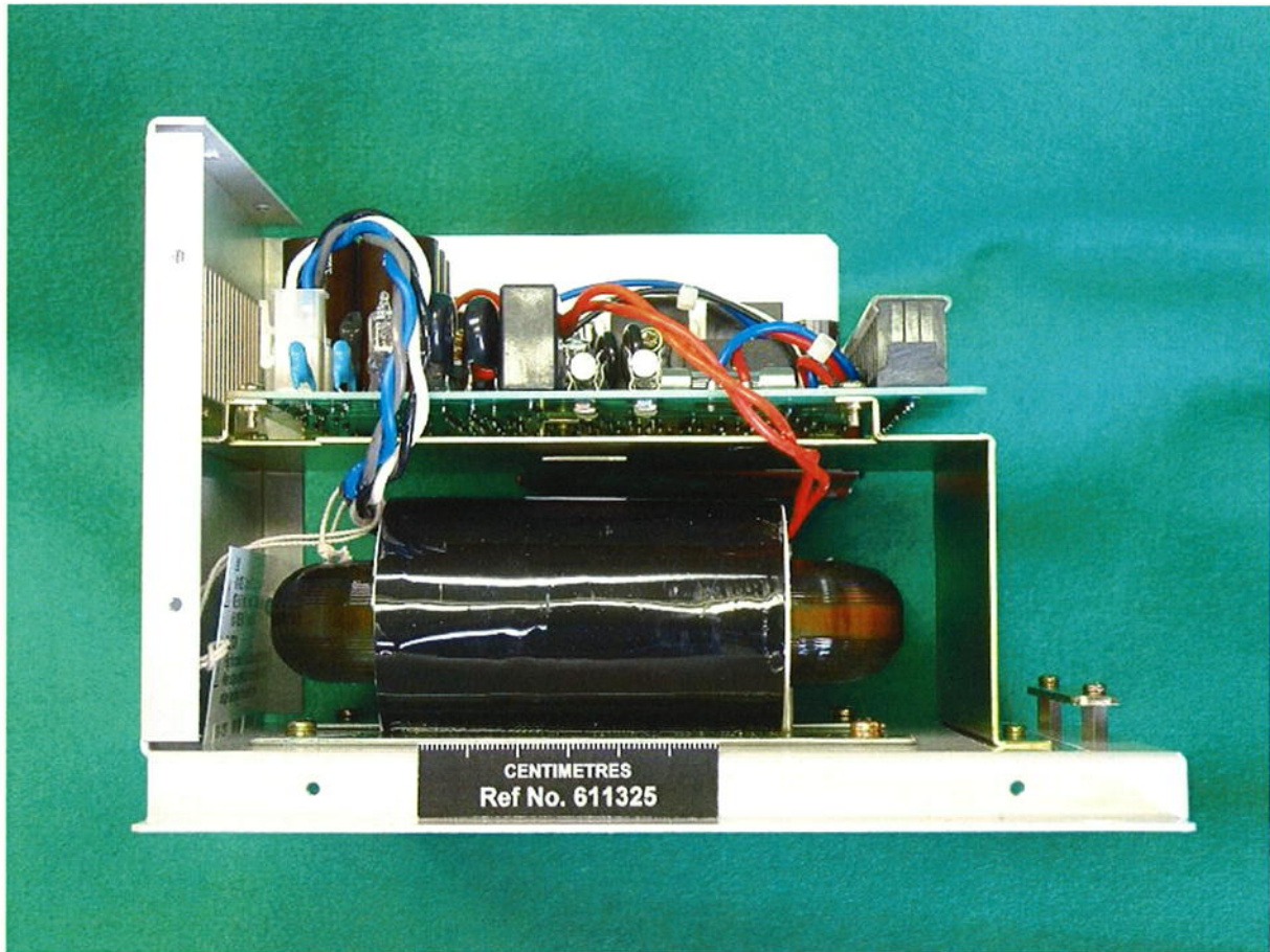
NBD-577B Power Supply – Internal view 2
