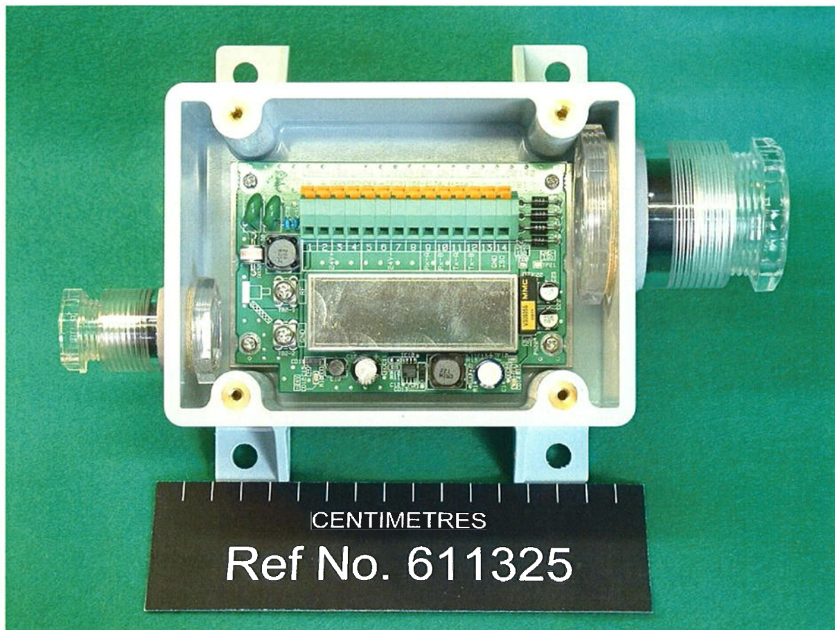
NQD-4382 Junction Box – Internal View
