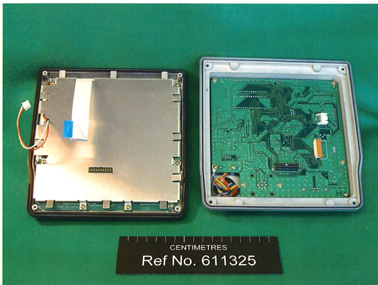
NCM-779 AIS Controller – Internal View 1
