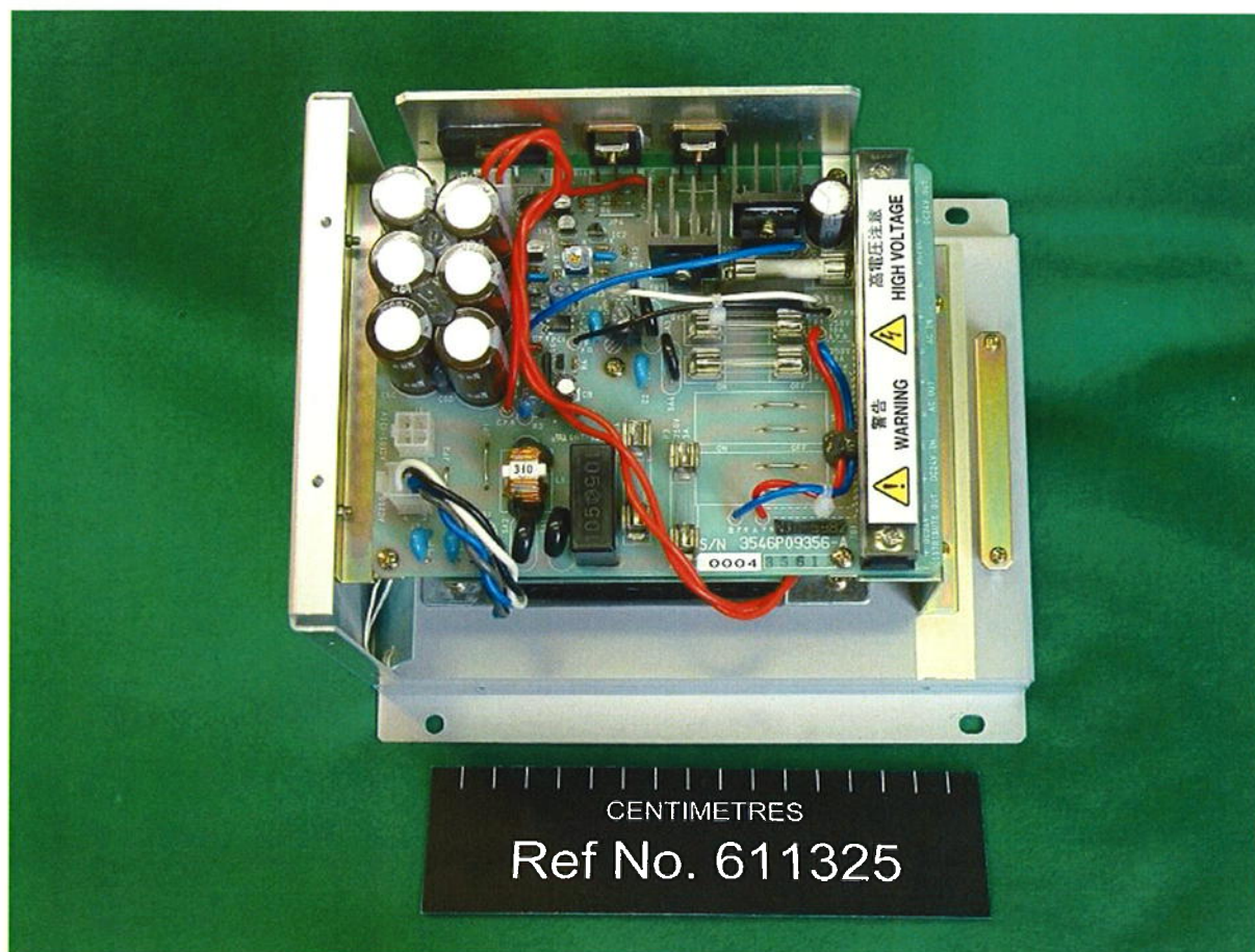
NBD-577B Power Supply – Internal view 1
