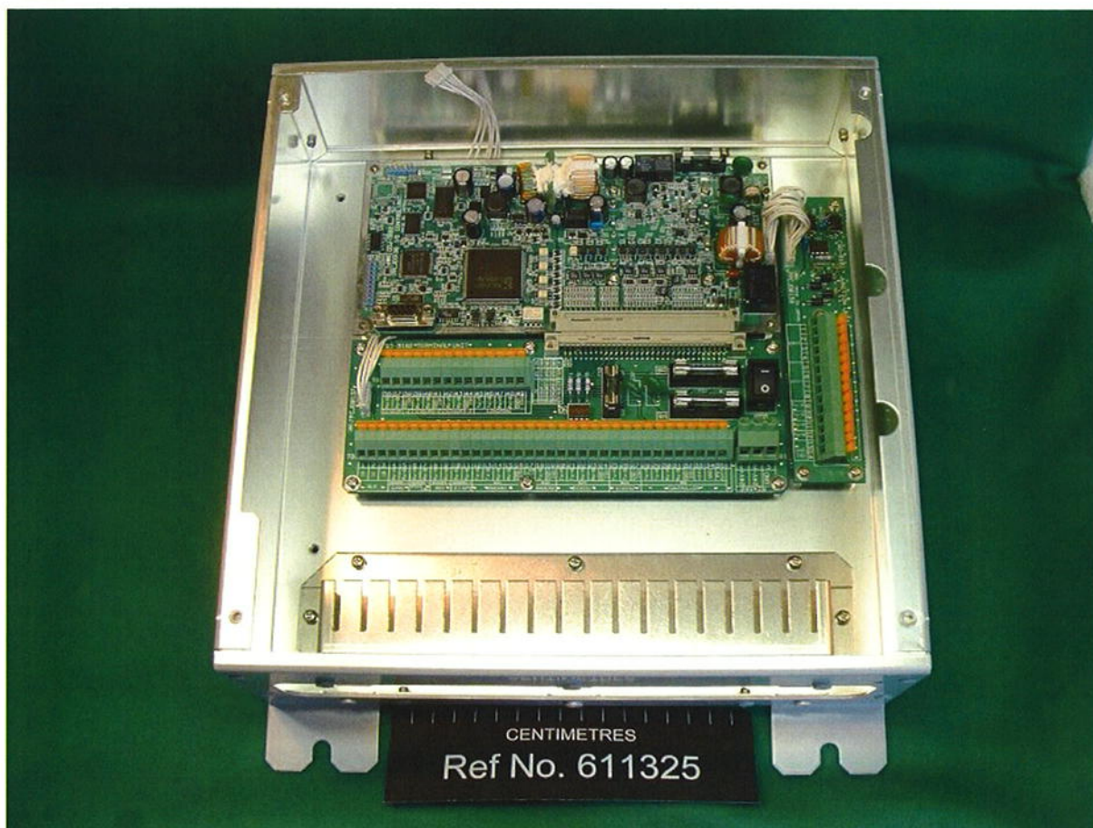
NQE-3182 Connection Box – Internal View
