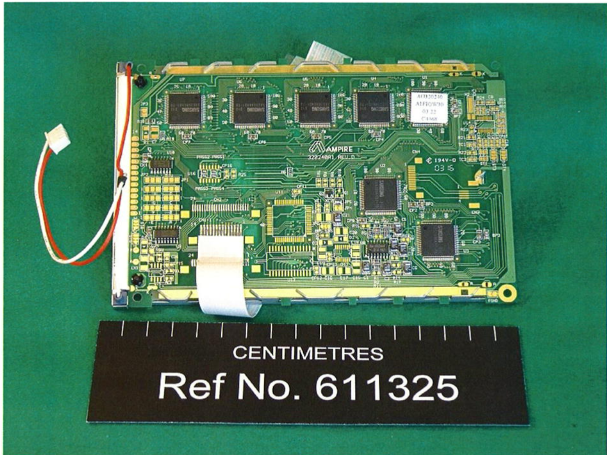
NCM-779 AIS Controller – Internal View 2
