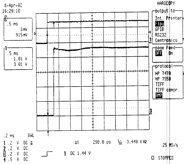
Figure x. Transmitter attack time and frequency characteristics at +55°C.
