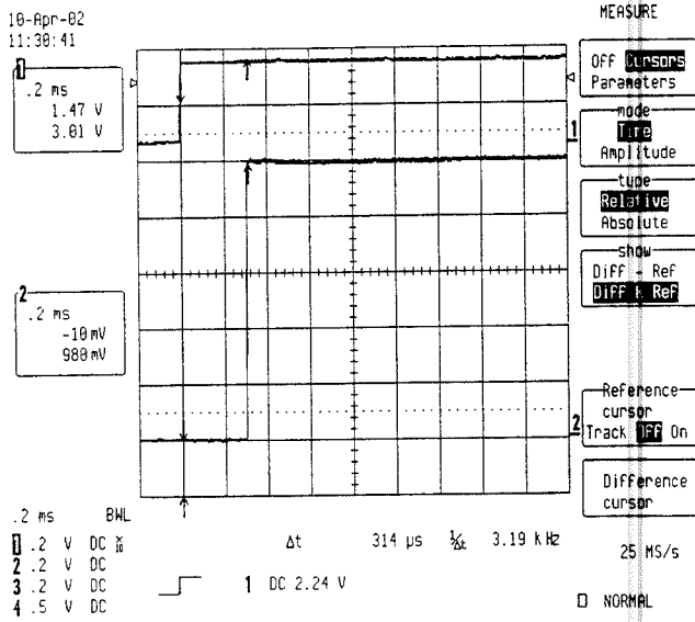
Figure x. Transmitter attack time and frequency characteristics at ambient temperature.
