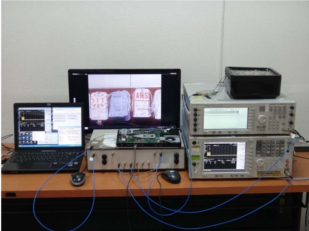
DFS Set-up Photo: Spectrum Analyzer, EUT and Radar Generator
