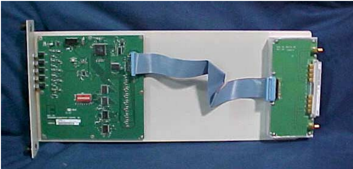
4.4.13 Inside view (sled assembly), Upstream/Downstream Output Switch Module
