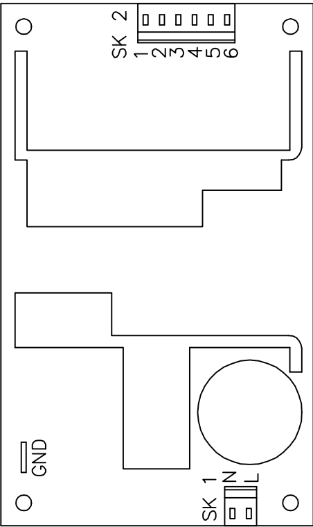
A4 & A6 DETAIL SWITCHING POWER SUPPLY PIN CONFIGURATION
