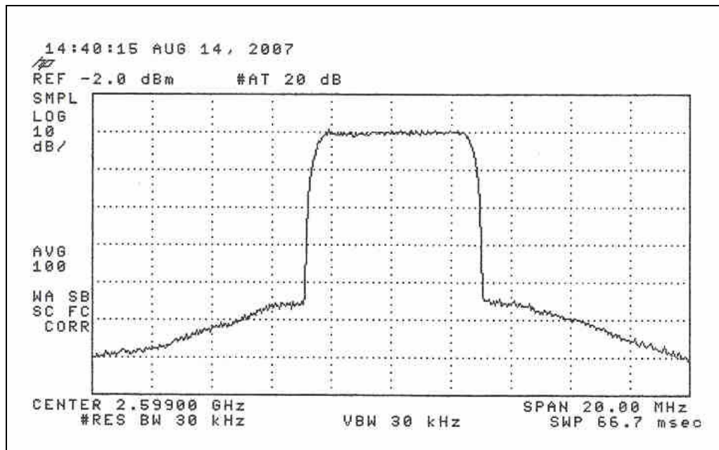
Figure 4-8. Conducted Spurious Emissions (before channel/band stop filter)
