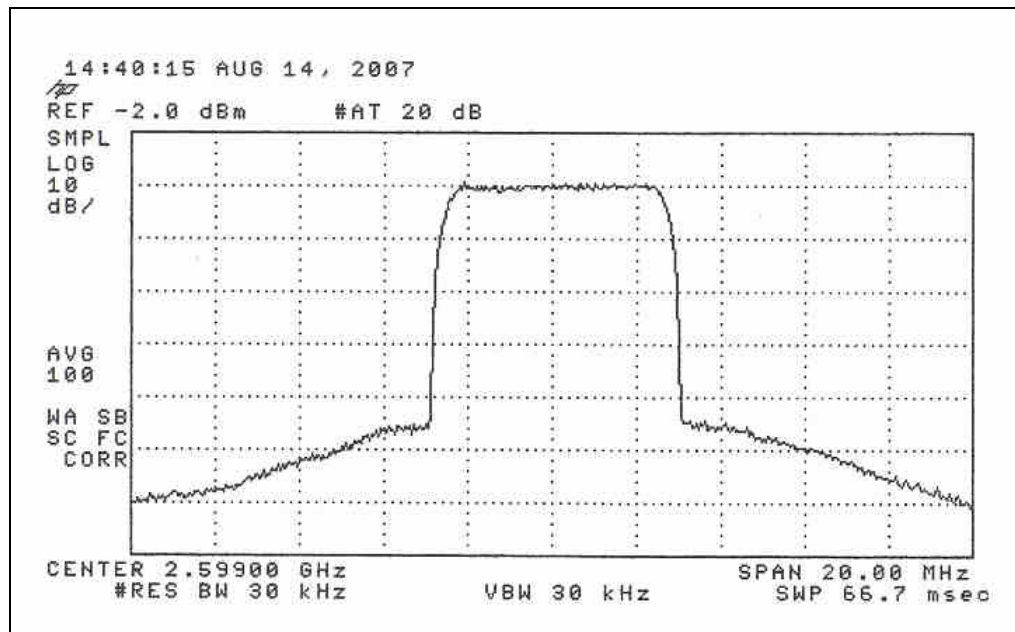
Figure 4-5. Channel Occupied Bandwidth
