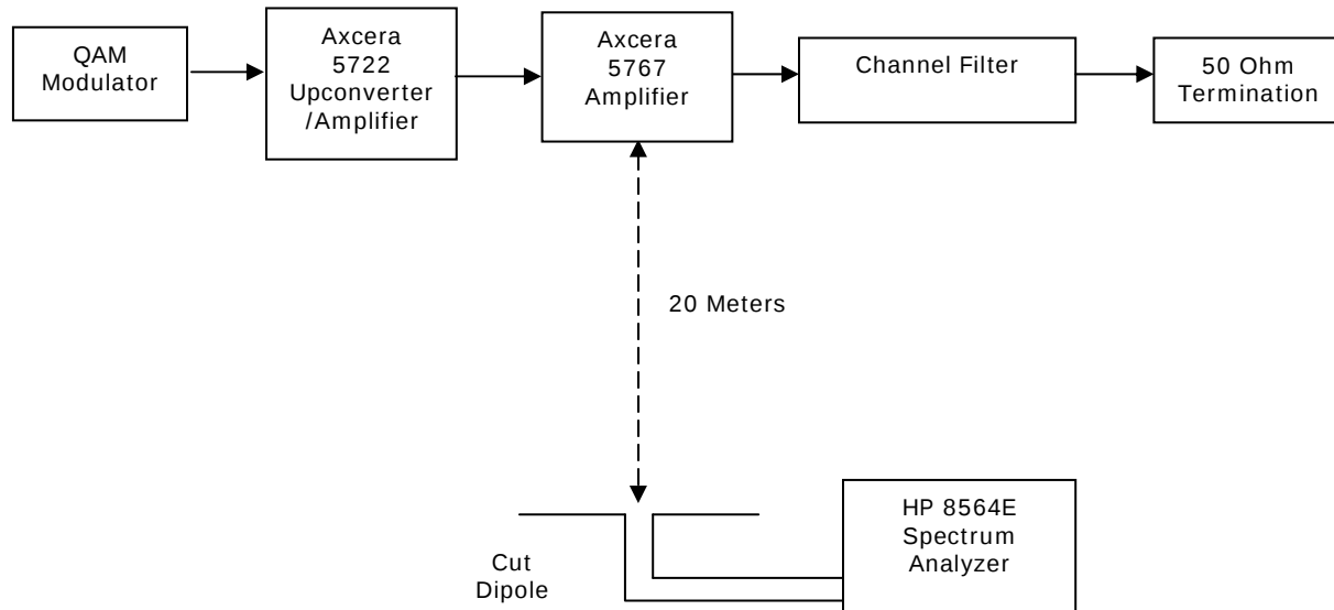
Figure 4-10. Test Setup for Measuring Radiated Emissions
