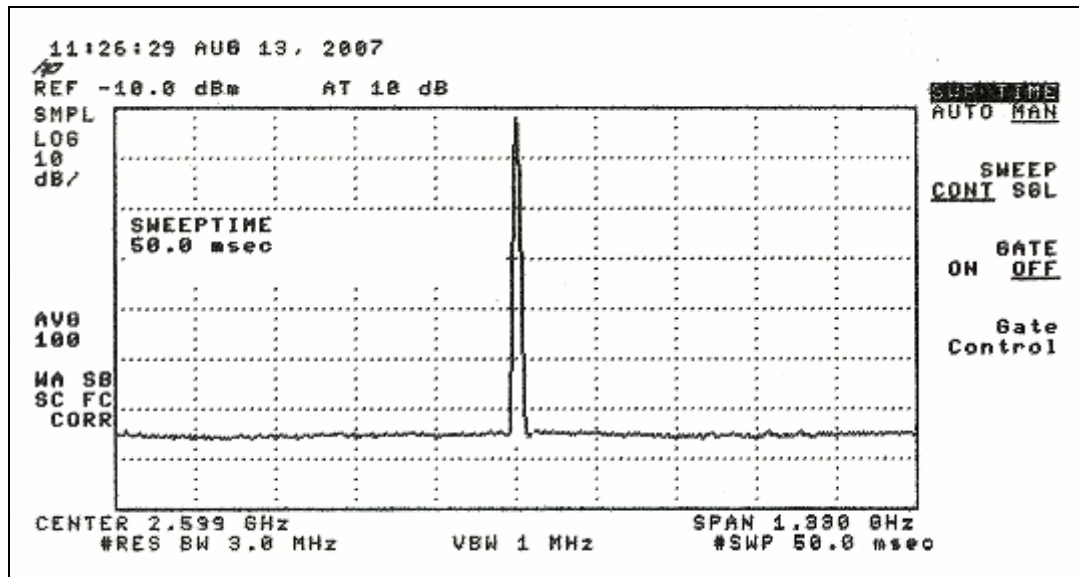
Figure 4-7. Products Above the -63 dB Noise Floor of the Spectrum Analyzer (1.330 GHz Span)
