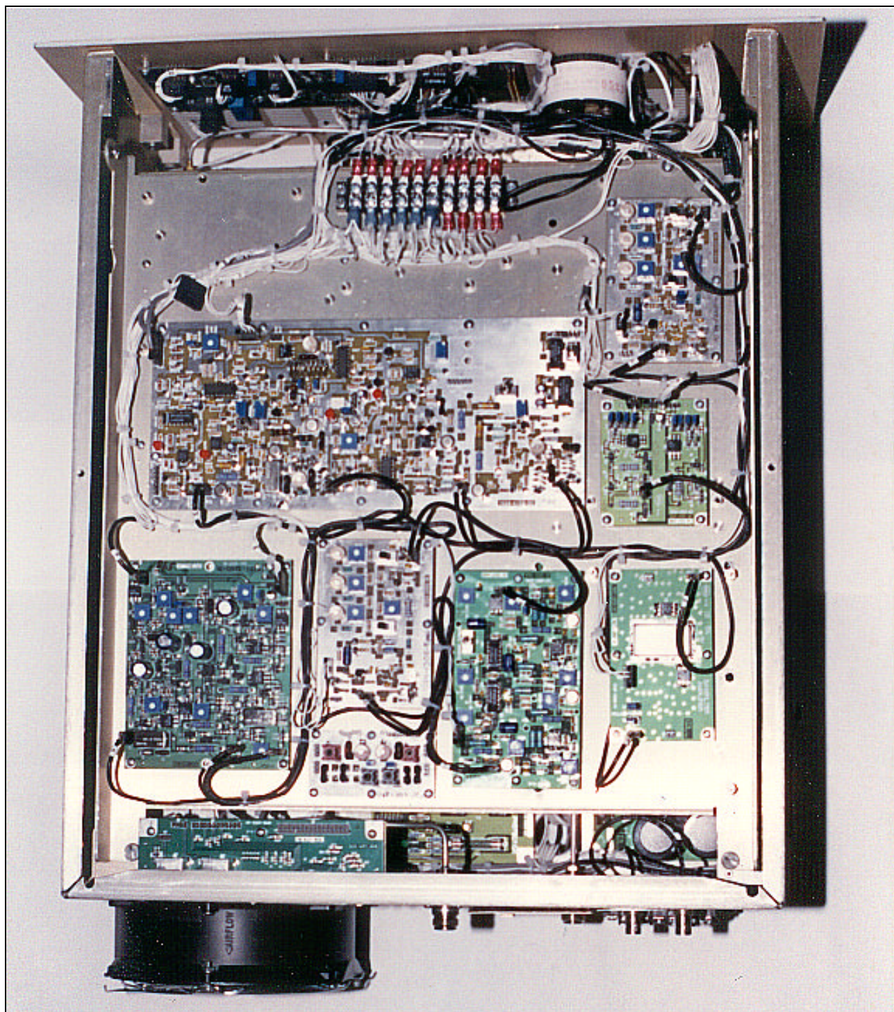
4.3.3 Top view, ITS-5523 Upconverter/Amplifier Tray (IF Section)
