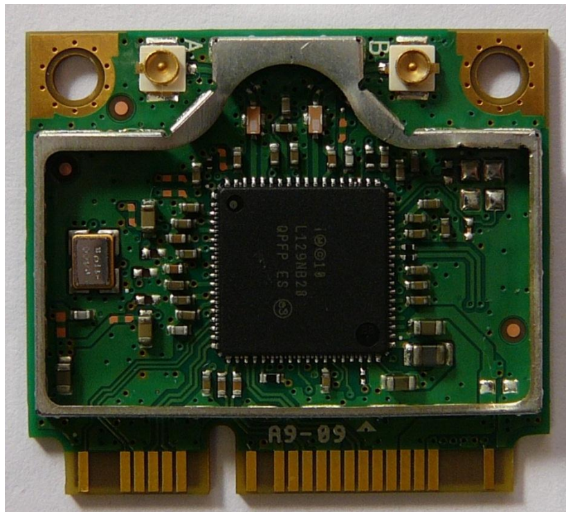
Top without shield
