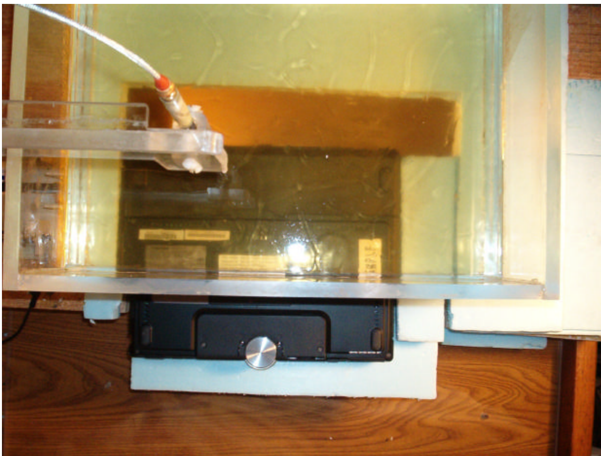
Fig. A. Top view photograph of the Toshiba PC for Configuration 1 of SAR testing. For this configuration, the cover with display screen is turned by 180° and folded back on the PC keyboard as for the PC tablet mode shown in Figs. 3-2 and 3-3 of the User's manual. Note that the underside of the keyboard is pressed against the base of the planar phantom for this configuration.
