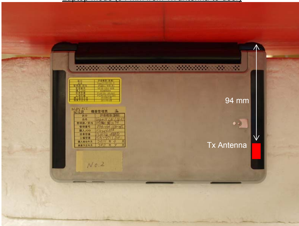
Laptop Mode (94 mm from Tx antenna-to-user)
