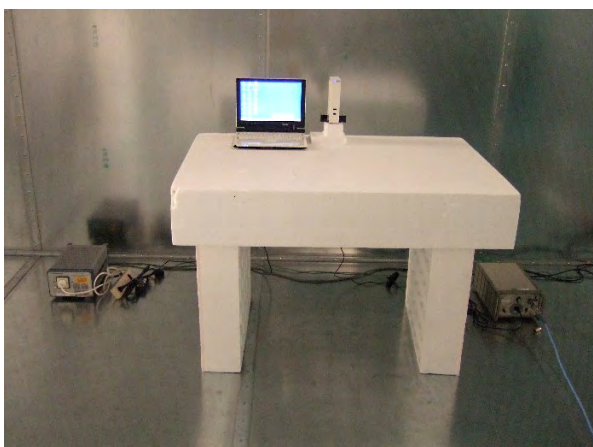
Test Configuration 4: AC conducted
