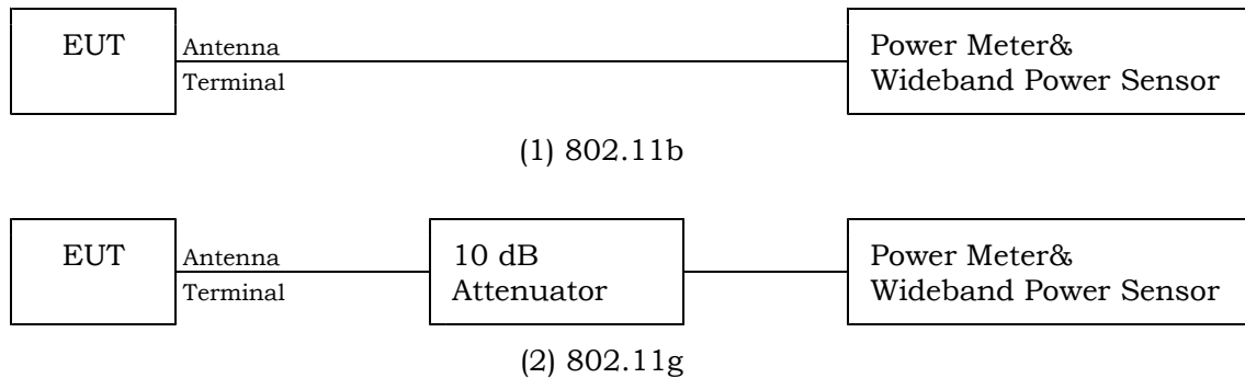
Fig.1 Transmitter Power Measurement
