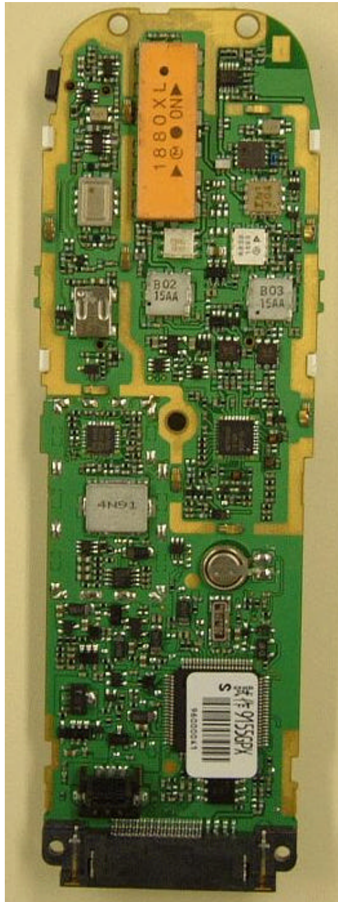
Handheld Portable MAIN Board (Back side , With shield cover removed) VCTCXO : KT16-ECV27L-19.680M-TA
