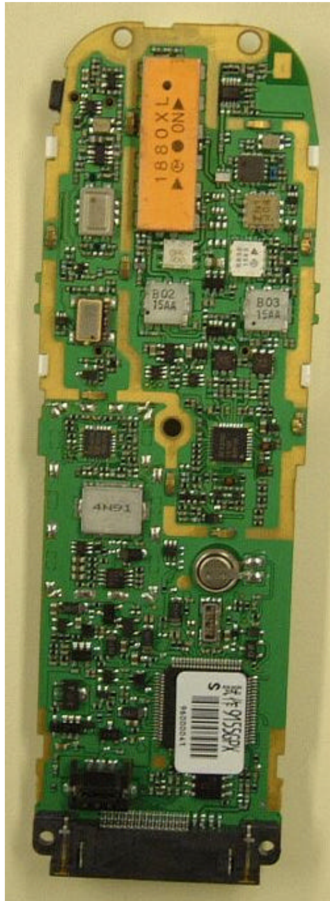
Handheld Portable MAIN Board (Back side , With shield cover removed) VCTCXO : DSA751HAD
