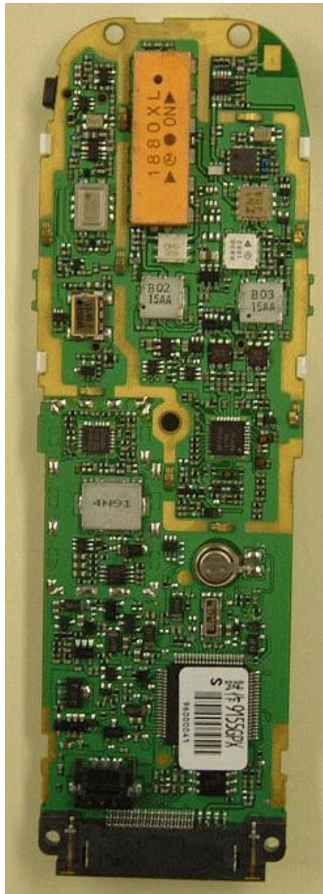
Handheld Portable MAIN Board (Back side , With shield cover removed) VCTCXO : VC-TCXO-204C2
