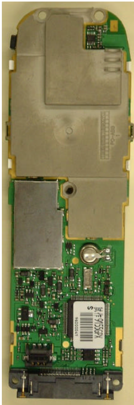
Handheld Portable MAIN Board (Back side , With shield cover)
