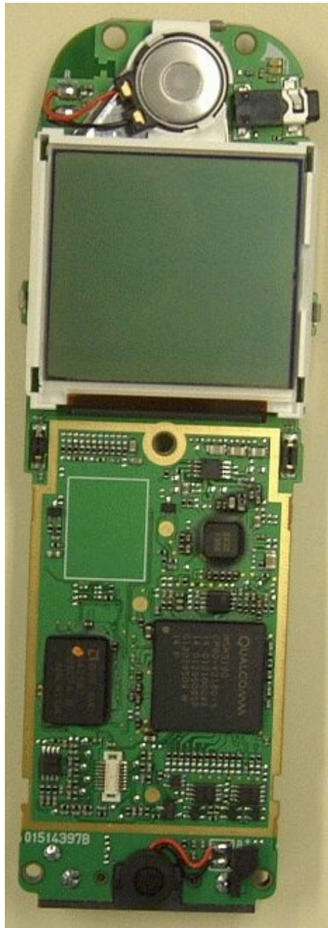
Handheld Portable MAIN Board (Front side , With Shield Cover Removed)
