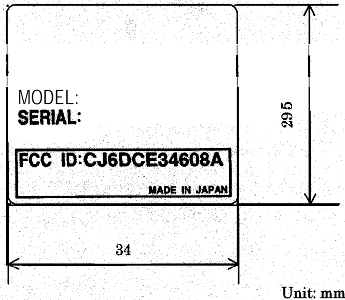
FCC ID Nameplate
