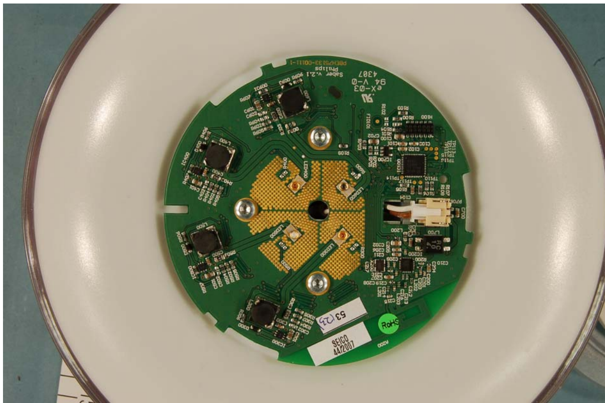
SABER – View of PCB
