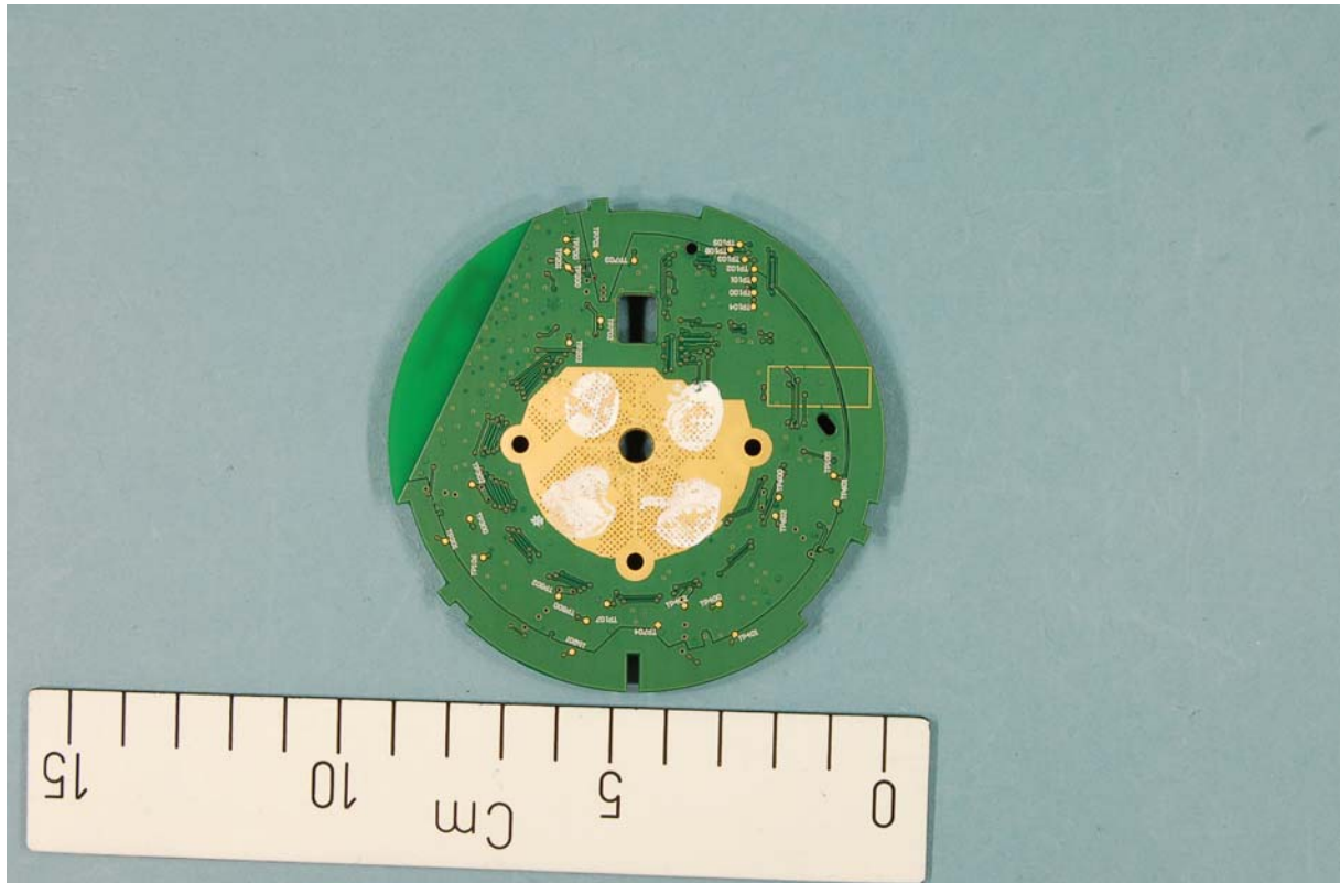
SABER – rear view of PCB
