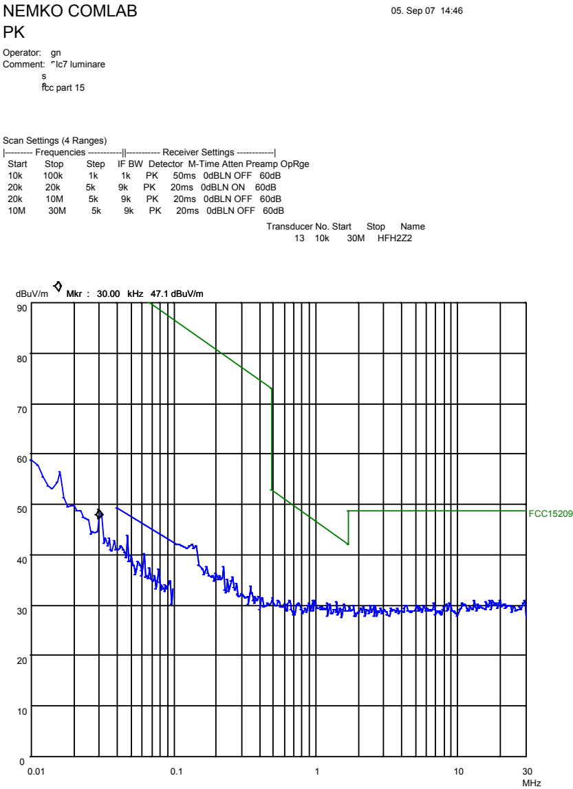
Luminaire - 10 kHz – 30MHz –radiated emission - (TX/RX mode)
