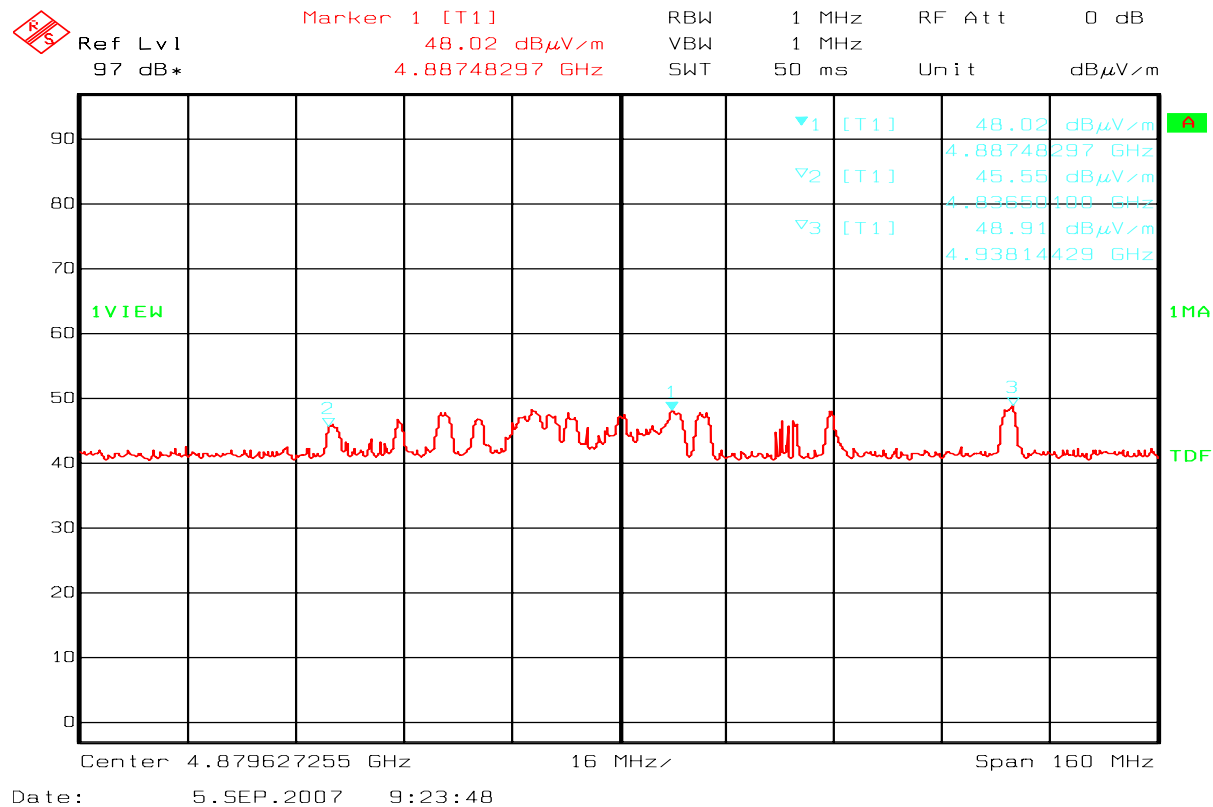
2 nd harmonic – Vertical Polarization
