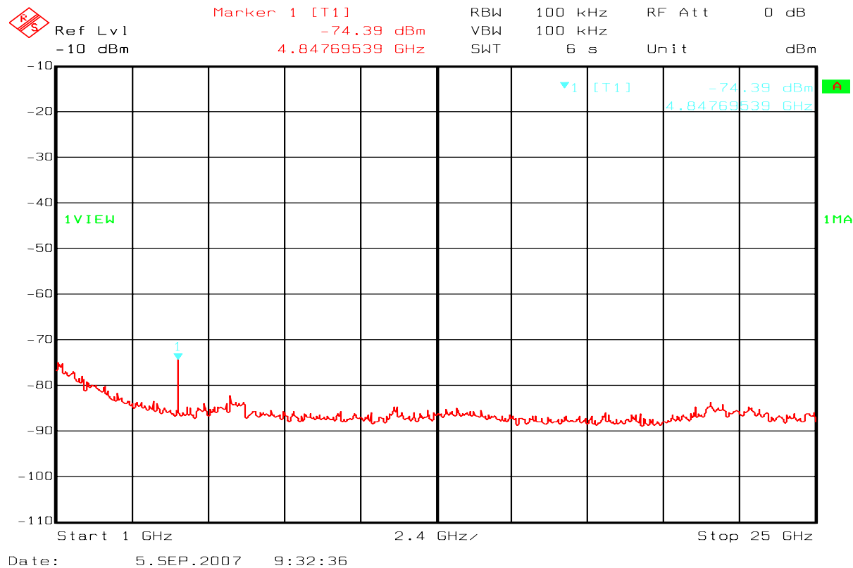
RX mode: Spurious scan 1 - 25 GHz (peak detector)
