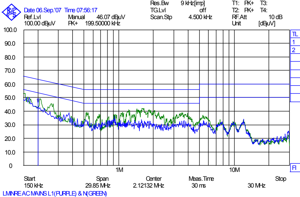
Conducted emission – In active mode
