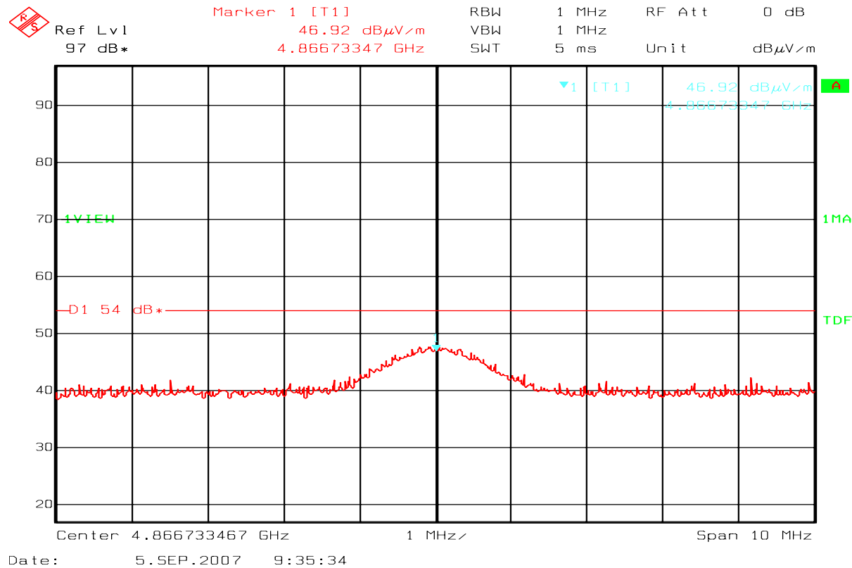
RX mode: 2 nd Harmonic (peak detector)
