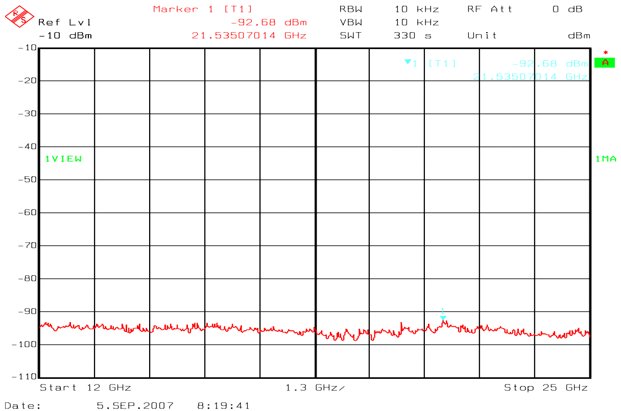
TX mode: Spurious scan 12 - 25 GHz (peak detector)
