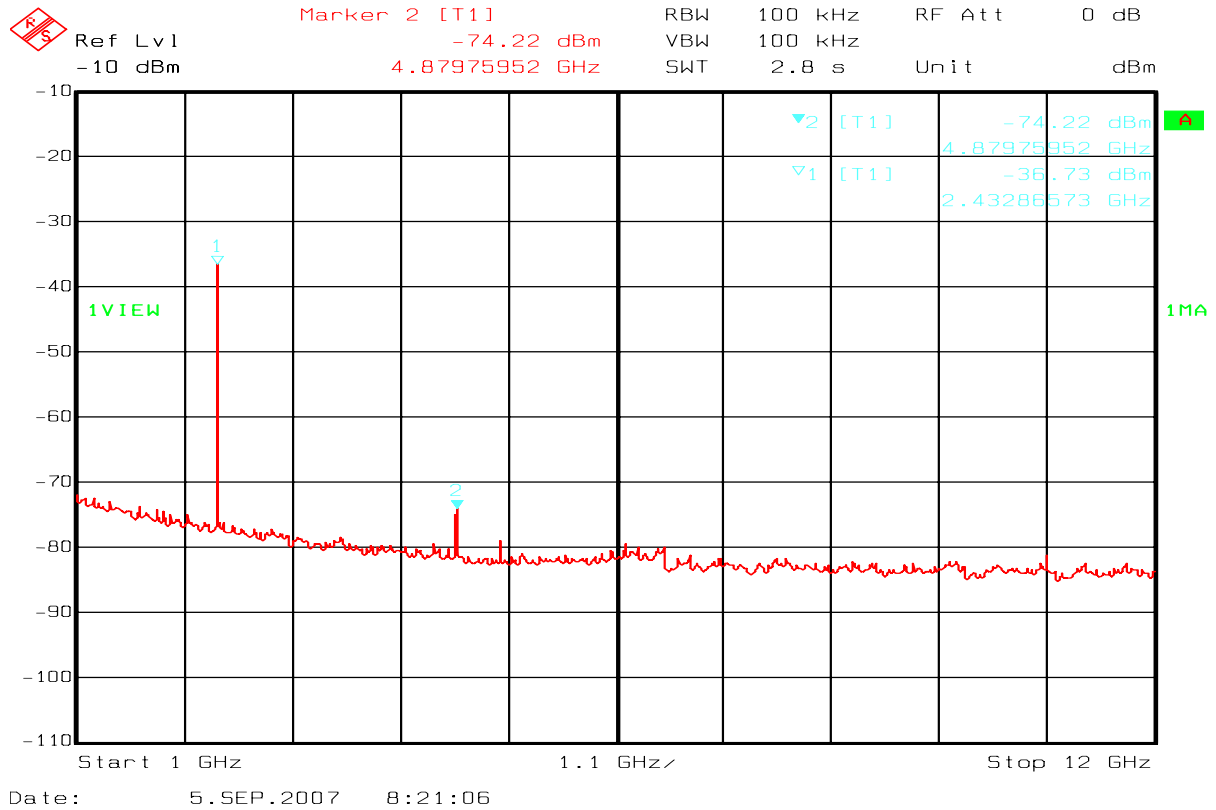
TX mode: Spurious scan 1 - 12 GHz (peak detector)
