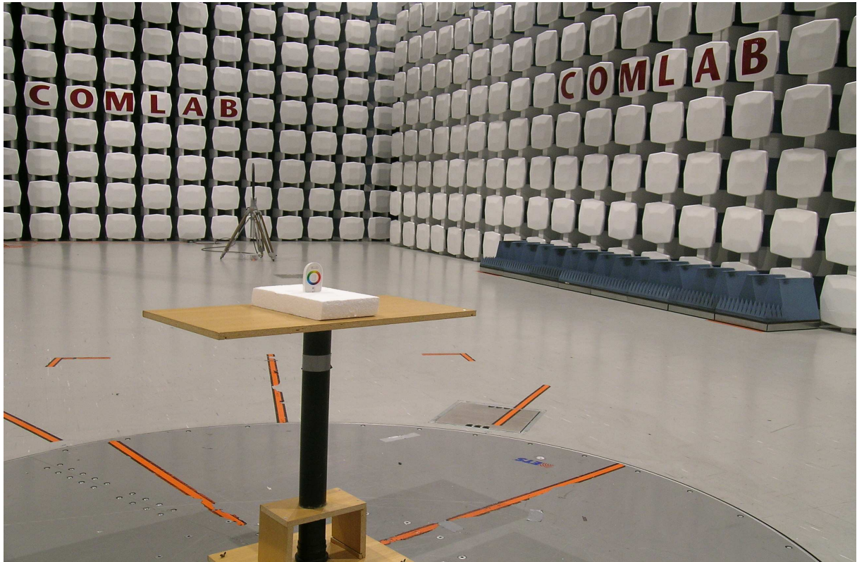
Radiated Emissions Test below 30MHz @10m
