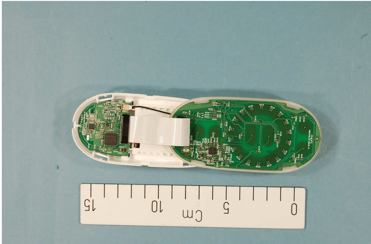
LC7 remote Control – Top view of PCB
