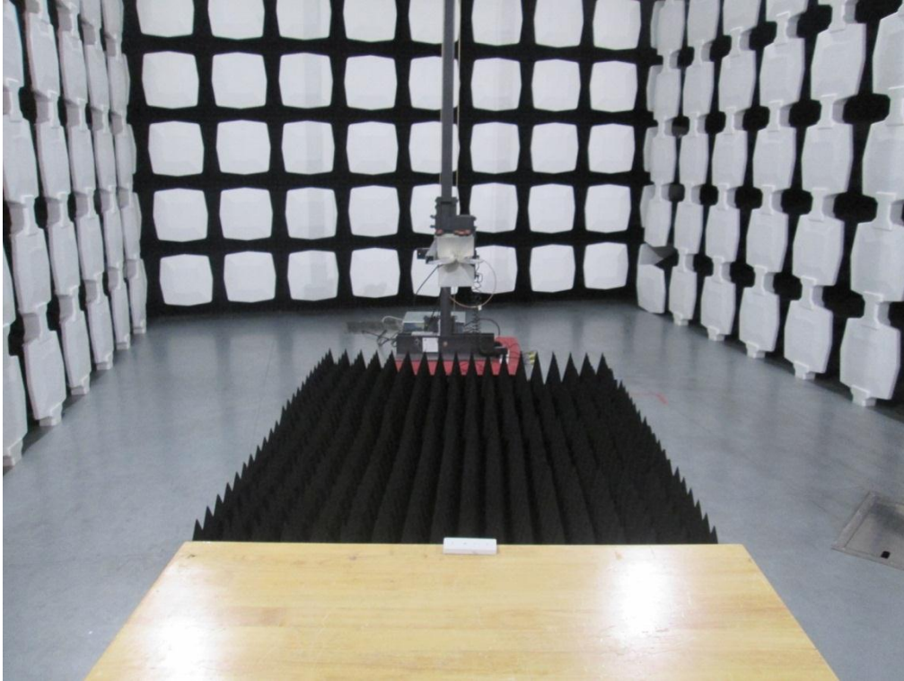
Figure 3 Radiated emission test setup (above 1 GHz)
