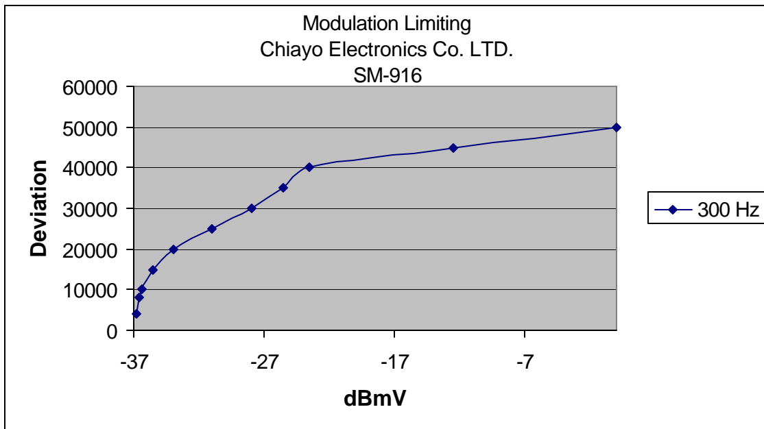
MODULATION LIMITING PLOT - 300 Hz
