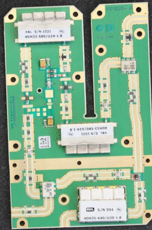
SCV-A113 Downconverter PCB 001335-2
