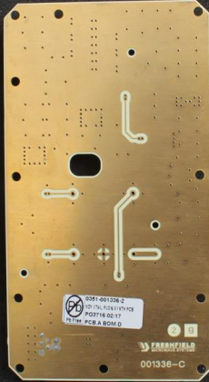
SCV-A113 Synth / PLO PCB 001336-2 (underside)
