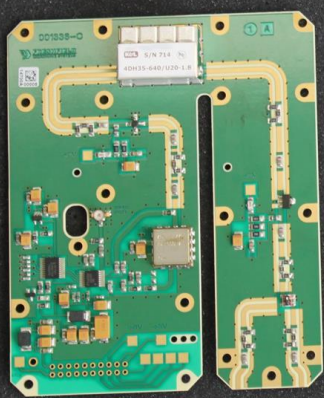
SCV-A113 Synth / PLO PCB 001336-1
