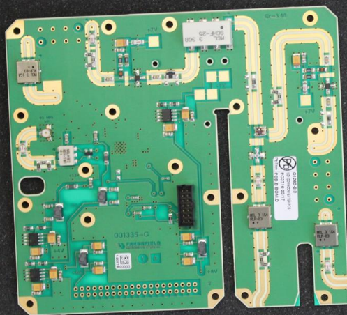
SCV-A113 Downconverter PCB 001335-1
