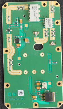
SCV-A113 Synth / PLO PCB 001336-2
