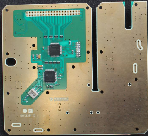
SCV-A113 Downconverter PCB 001335-1 (underside)
