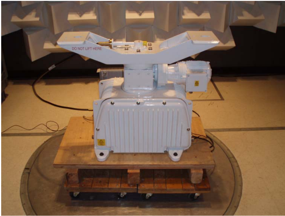
Cabinet Radiation setup photo
