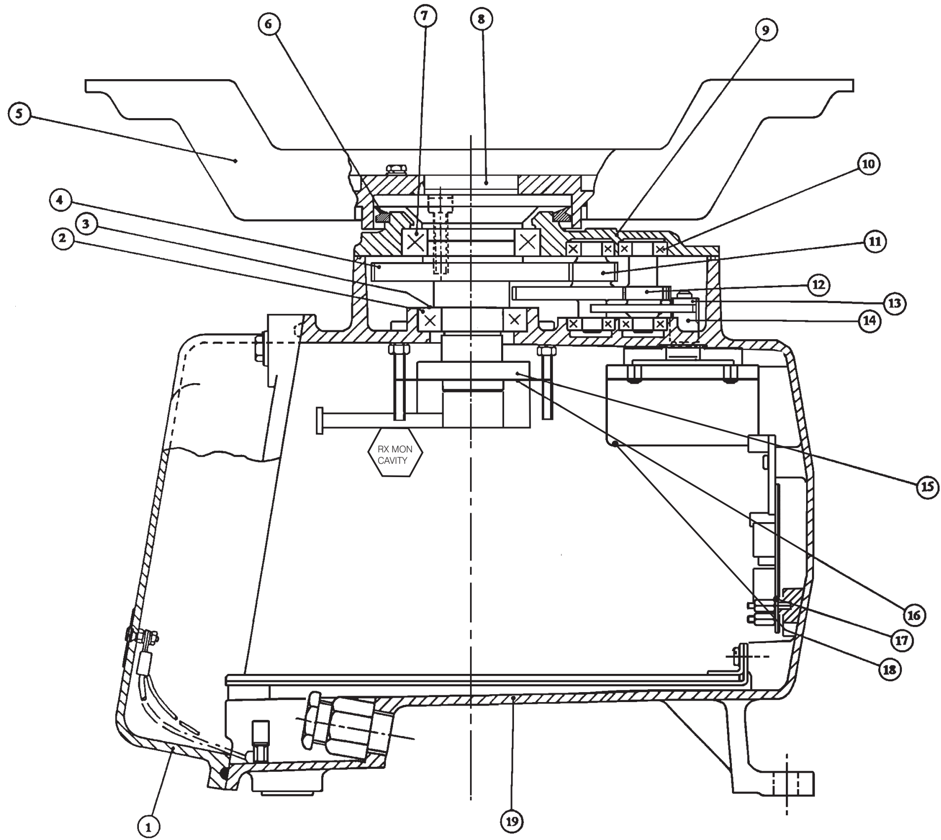
Turning Mechanism: Main Assemblies
