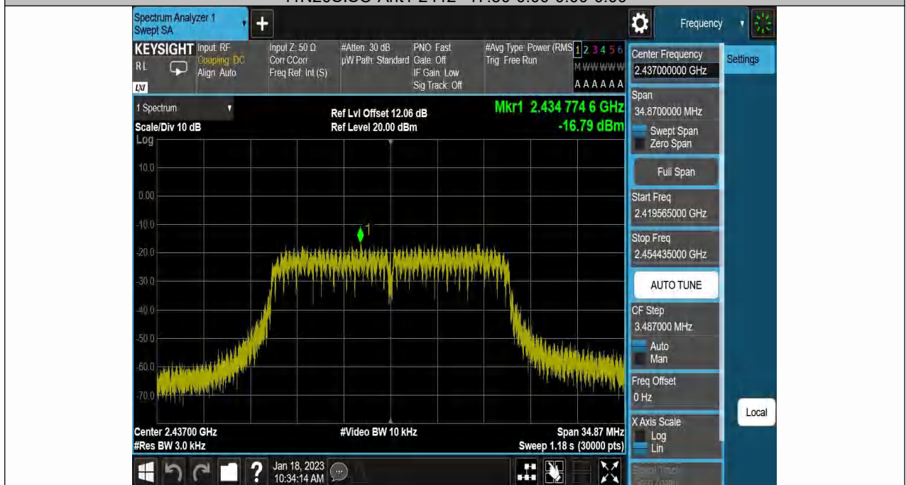
11N20SISO-Ant1-2437--16.79-0.00-0.00-0.00
