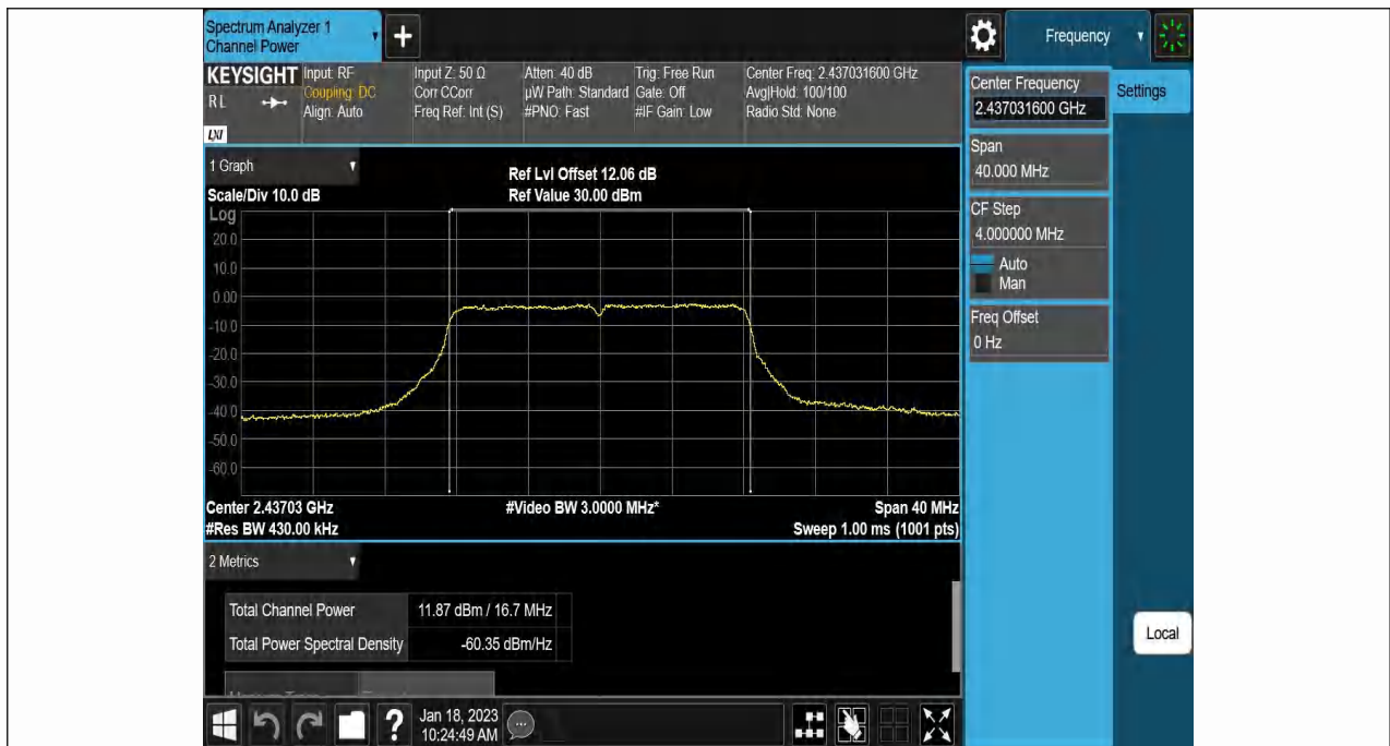
11G-Ant1-2437-----11.87-100.00-0.00
