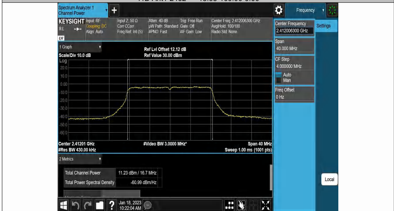
11G-Ant1-2412-----11.23-100.00-0.00
