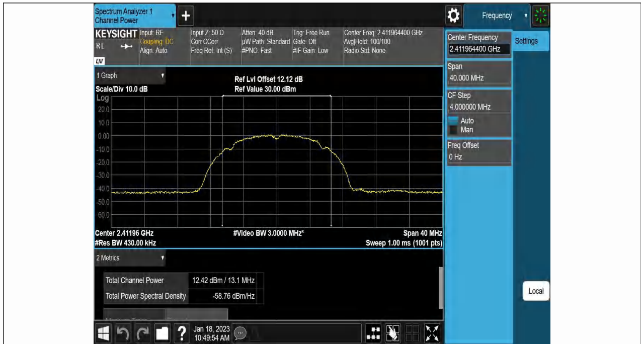
11B-Ant1-2412-----12.42-100.00-0.00
