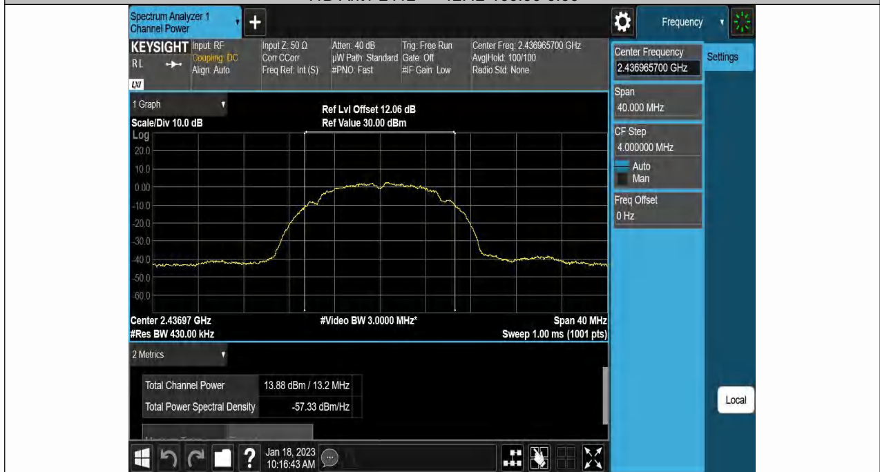
11B-Ant1-2437-----13.88-100.00-0.00
