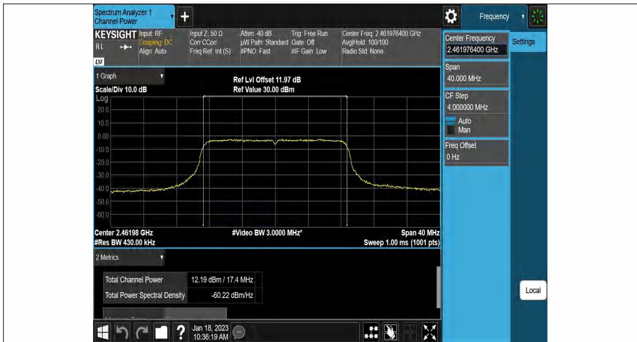
11N20SISO-Ant1-2462-----12.19-100.00-0.00
