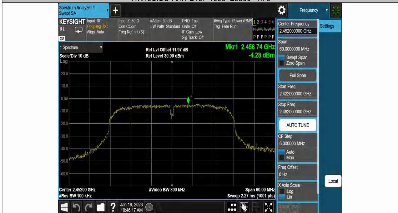
11N40SISO-Ant1-2452-0~Reference--4.28
