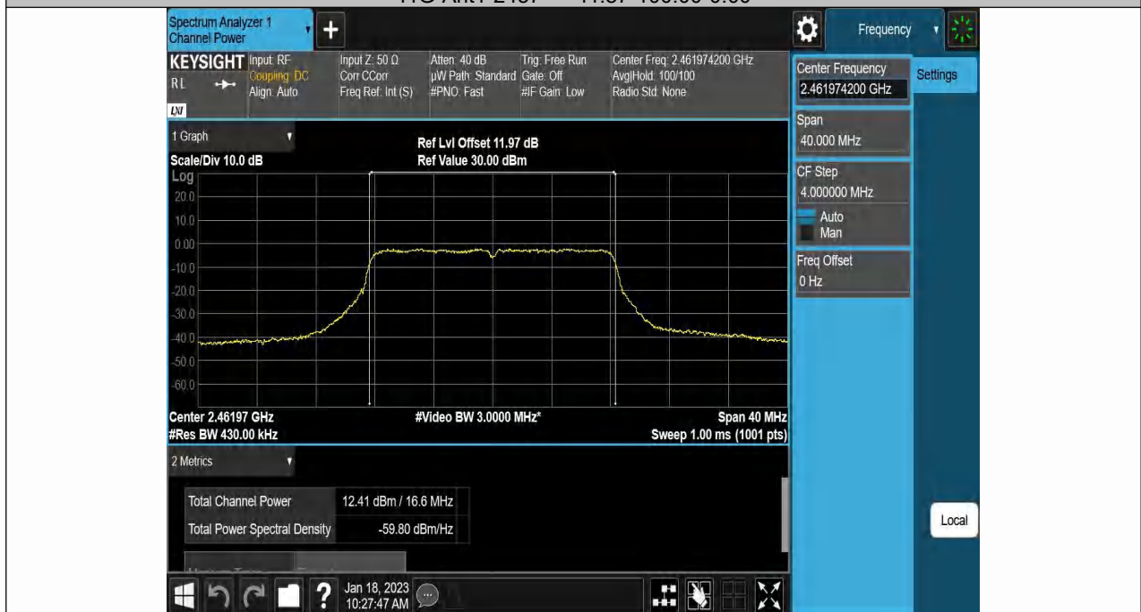
11G-Ant1-2462-----12.41-100.00-0.00
