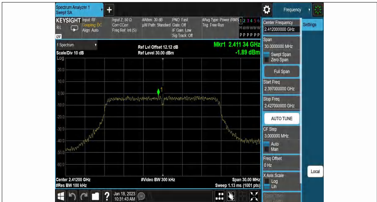
11N20SISO-Ant1-2412-0~Reference--1.89
