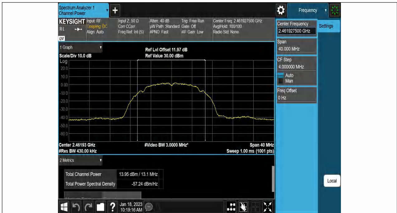
11B-Ant1-2462-----13.95-100.00-0.00
