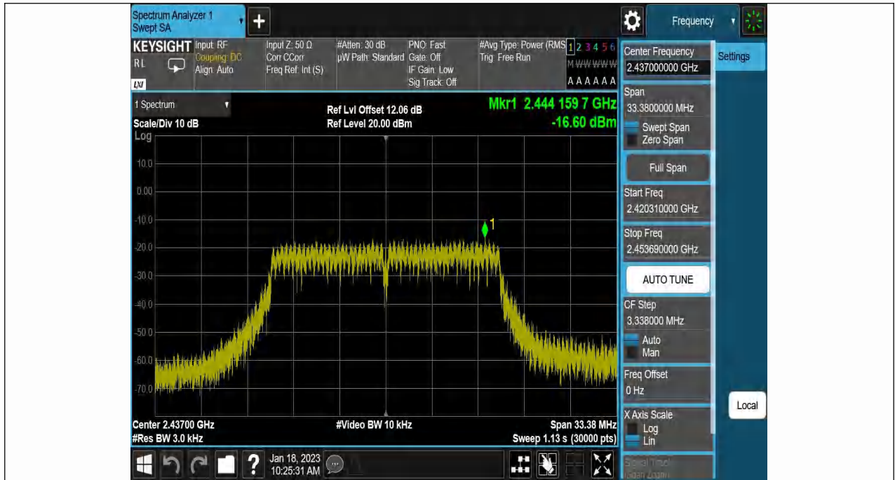
11G-Ant1-2437--16.60-0.00-0.00-0.00
