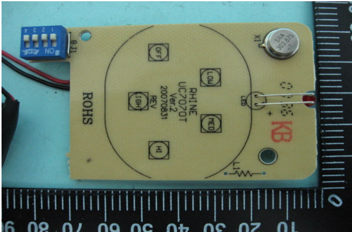
Solder View of EUT
