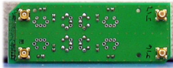
Figure 8 45324540 PCB Bottom Side View
