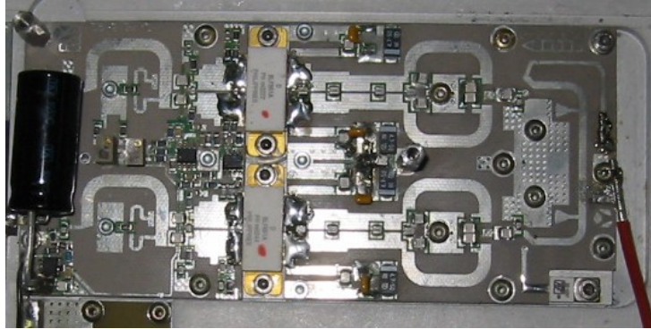
Figure 19 45324585 PCB Top Side View
