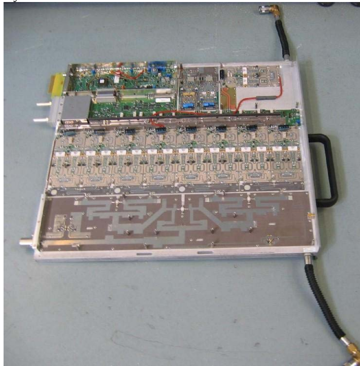
Figure 13 Amplifier Top Side View
