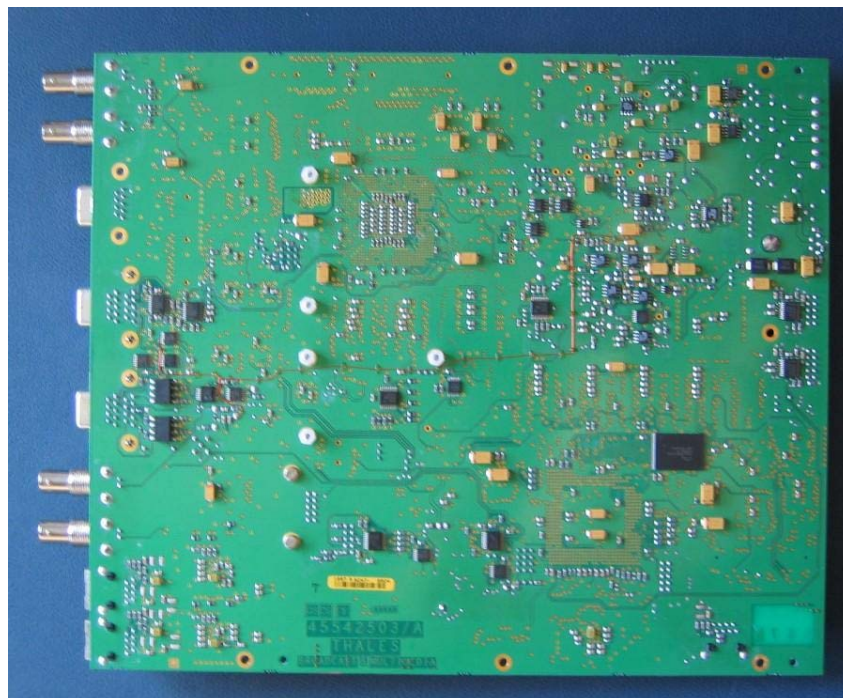
Figure 4 45324527.01 PCB Bottom Side View
