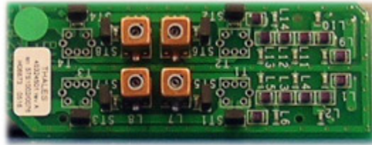
Figure 7 45324540 PCB Top Side View
