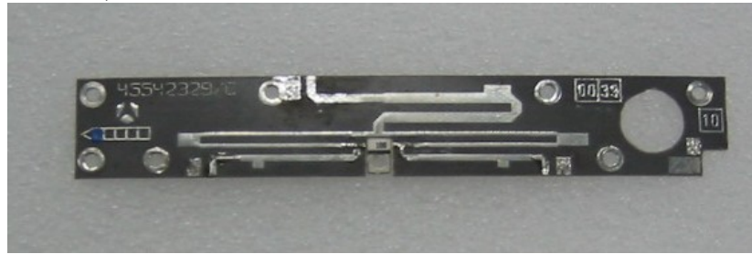
Figure 15 45324270 PCB Top Side View
