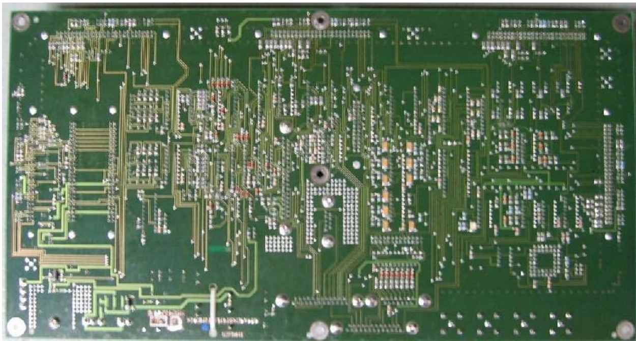
Figure 24 45324499 PCB Bottom Side View
