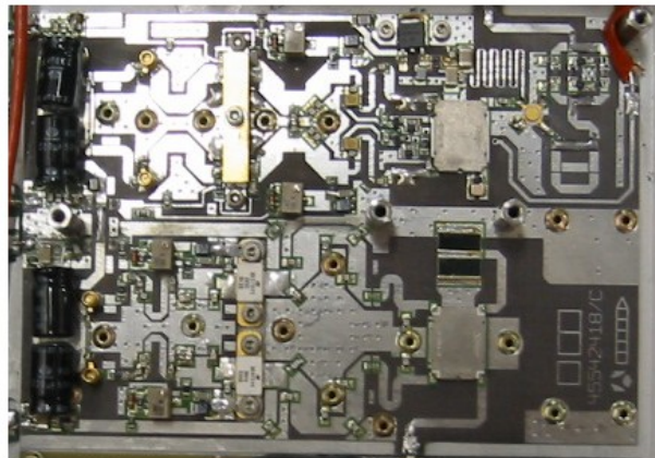
Figure 17 45324403 PCB Top Side View
