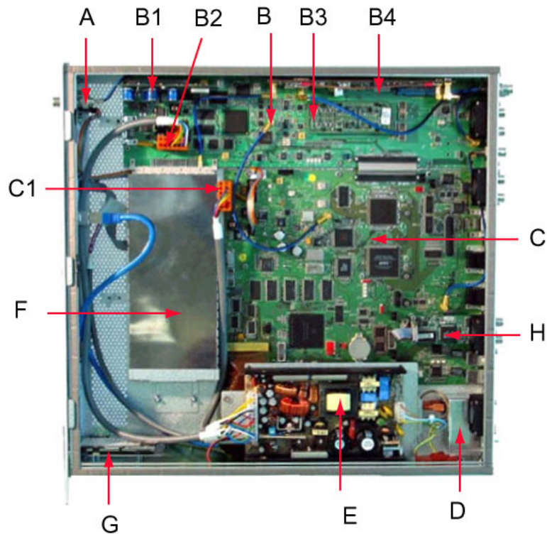
Figure 5 Exciter (top view)
