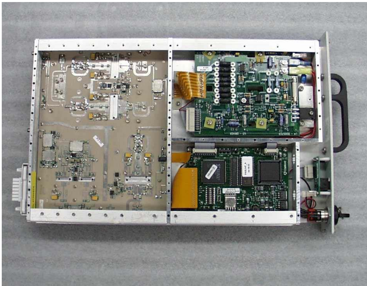
Figure 8 Power amp plug-in
