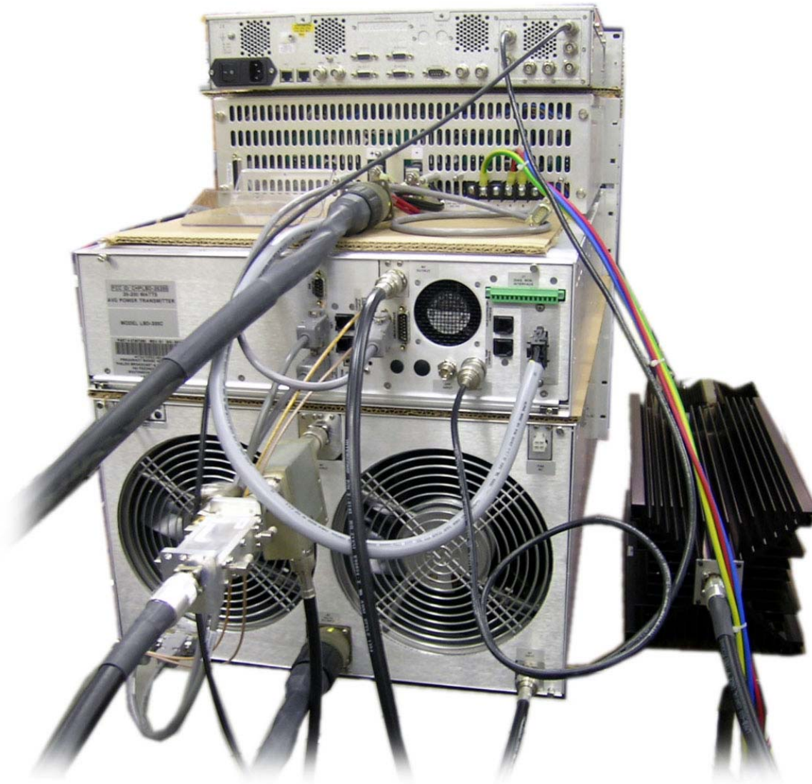
Figure 4 Transmitter rear view (full)
