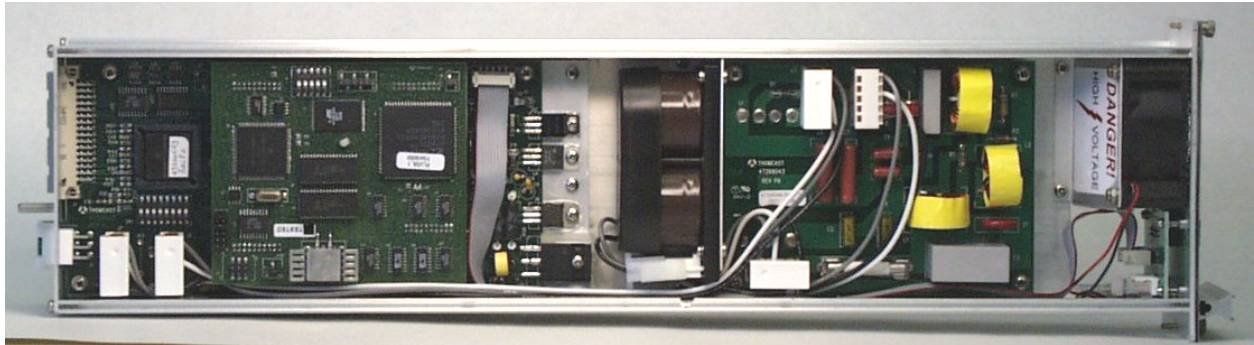
Figure 6 Power supply plug-in
