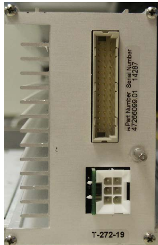
Figure 10: Power supply plug-in module front panel. Figure 11: Power supply plug-in module rear panel.
