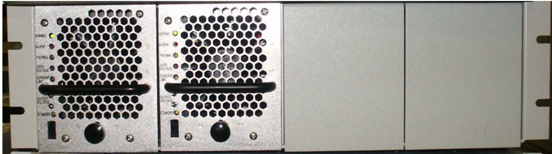
Figure 4 Front-end 48VDC rectifier system (front view)
