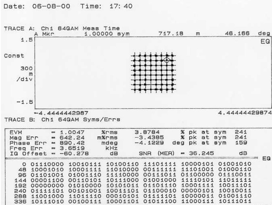
PLOT 1: Demodulation performance of the 64 QAM transmitter.
