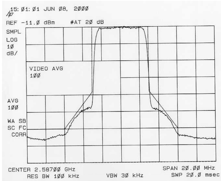
PLOT 5: Occupied bandwidth of the 64 QAM transmitter.
