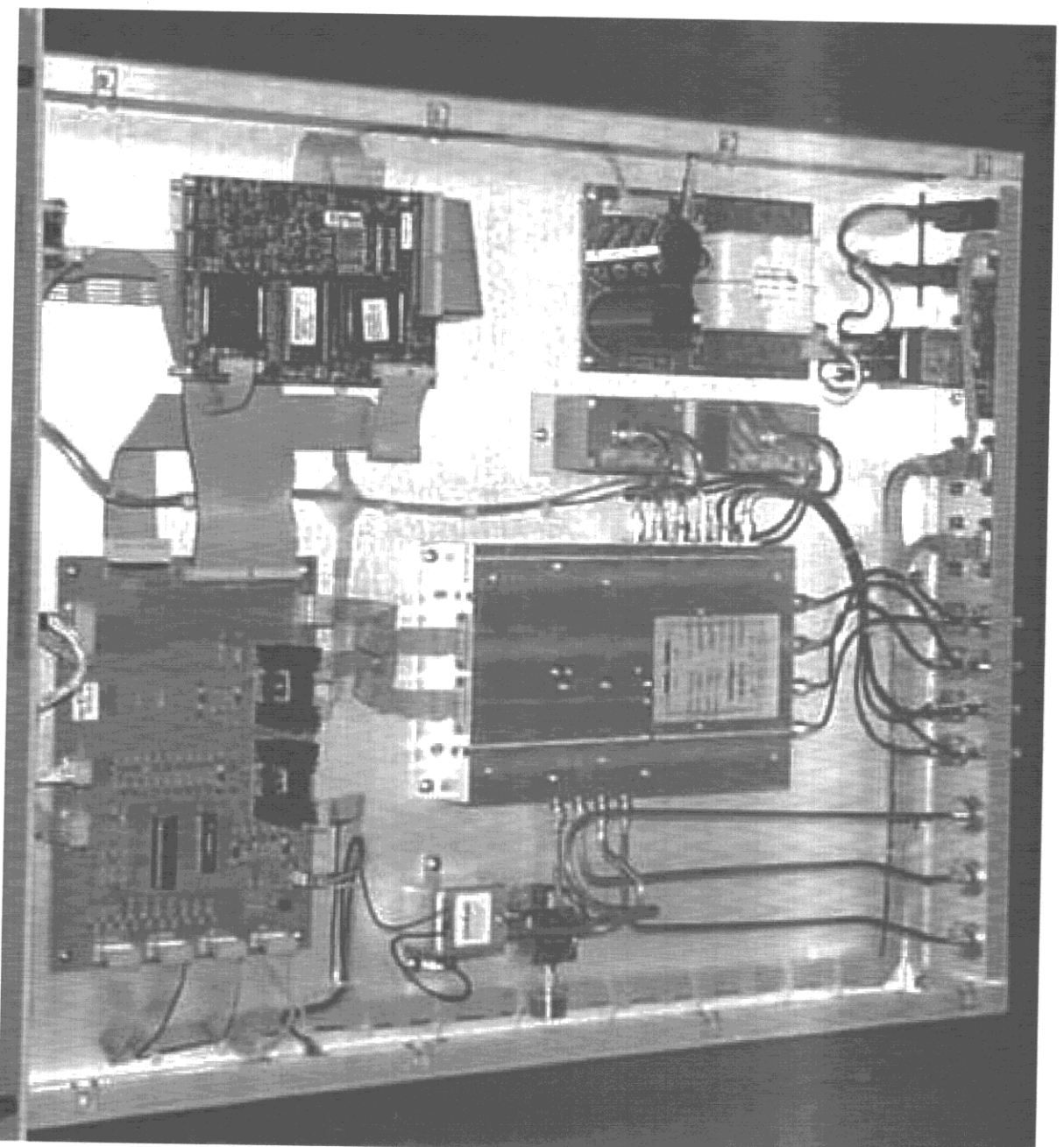
SWITCH AND CONTROL DRAWER TOP VIEW
