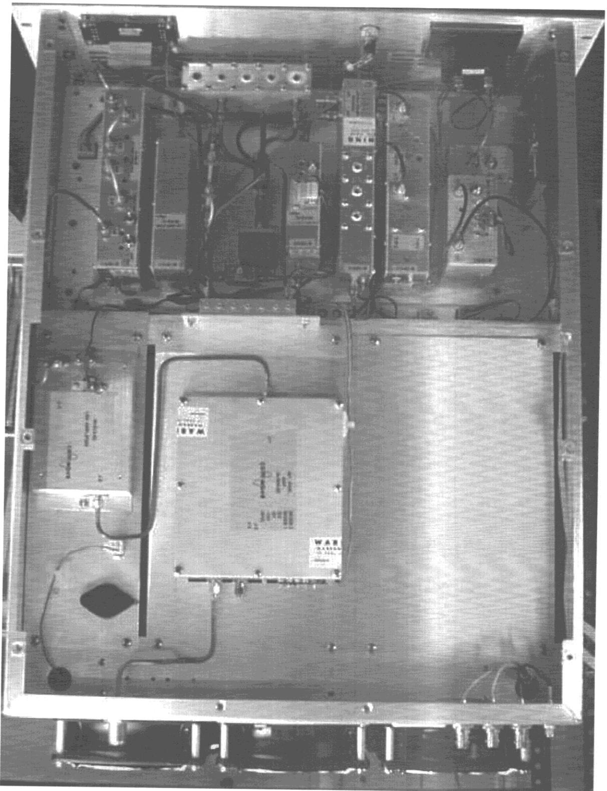
SBM-500A VHF/UHF TO \mu W UPCONVERTER (DRIVER) TOP VIEW
