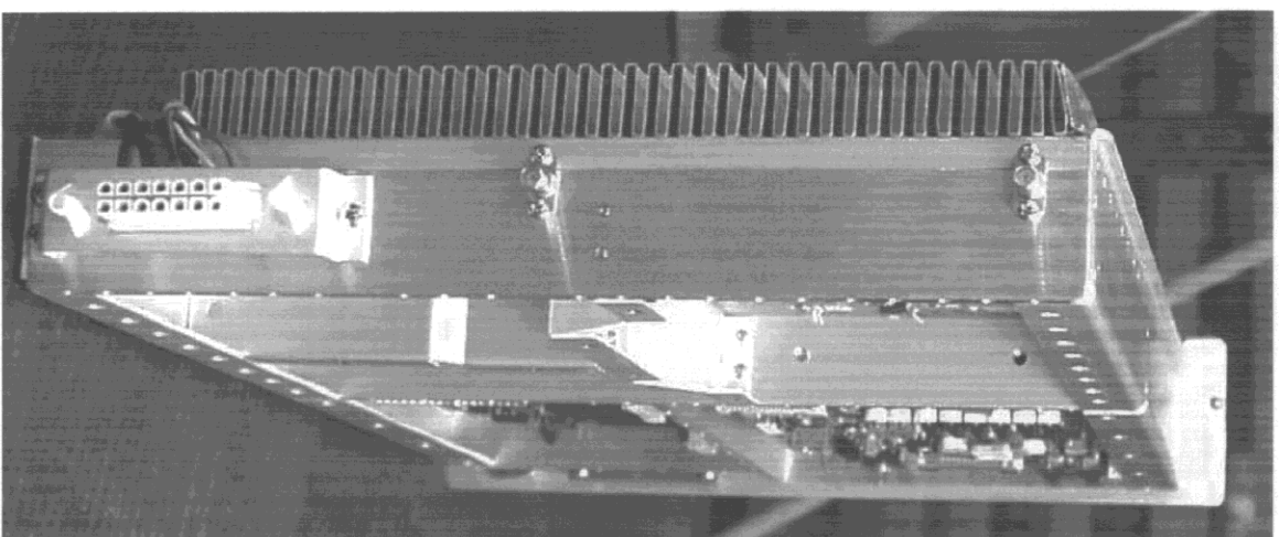
SBM-250A POWER AMPLIFIER SEGMENT FRONT AND REAR VIEWS
