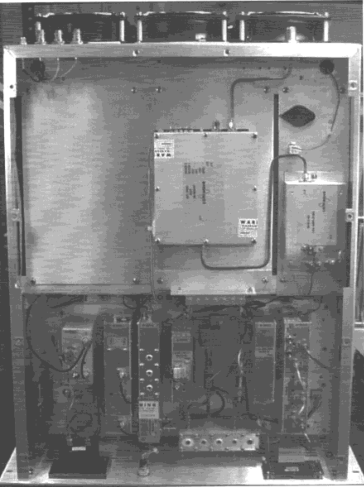
SBM-250A VHF/UHF TO \mu W UPCONVERTER (DRIVER) TOP VIEW
