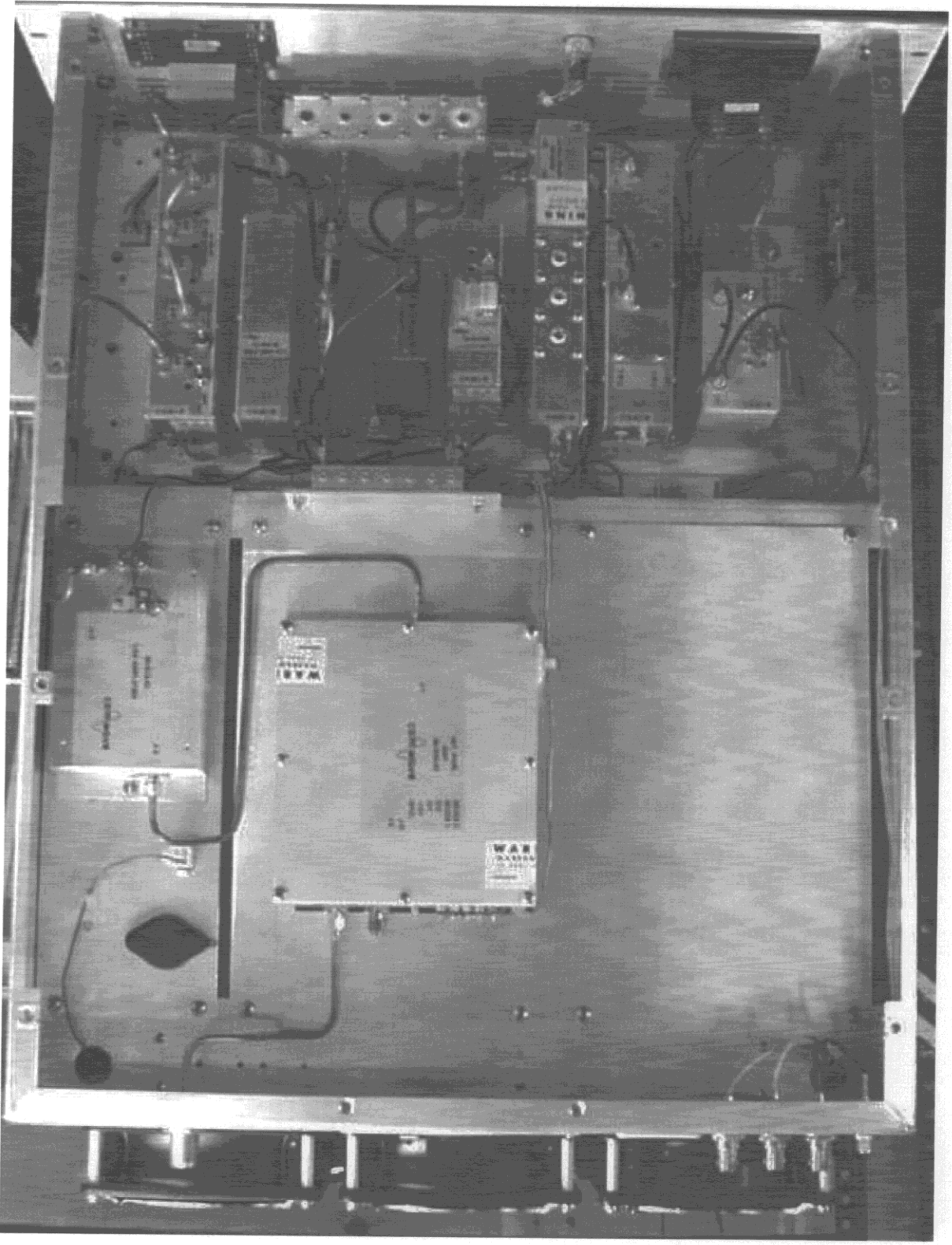
SBM-1000A VHF/UHF TO \mu W UPCONVERTER (DRIVER) TOP VIEW
