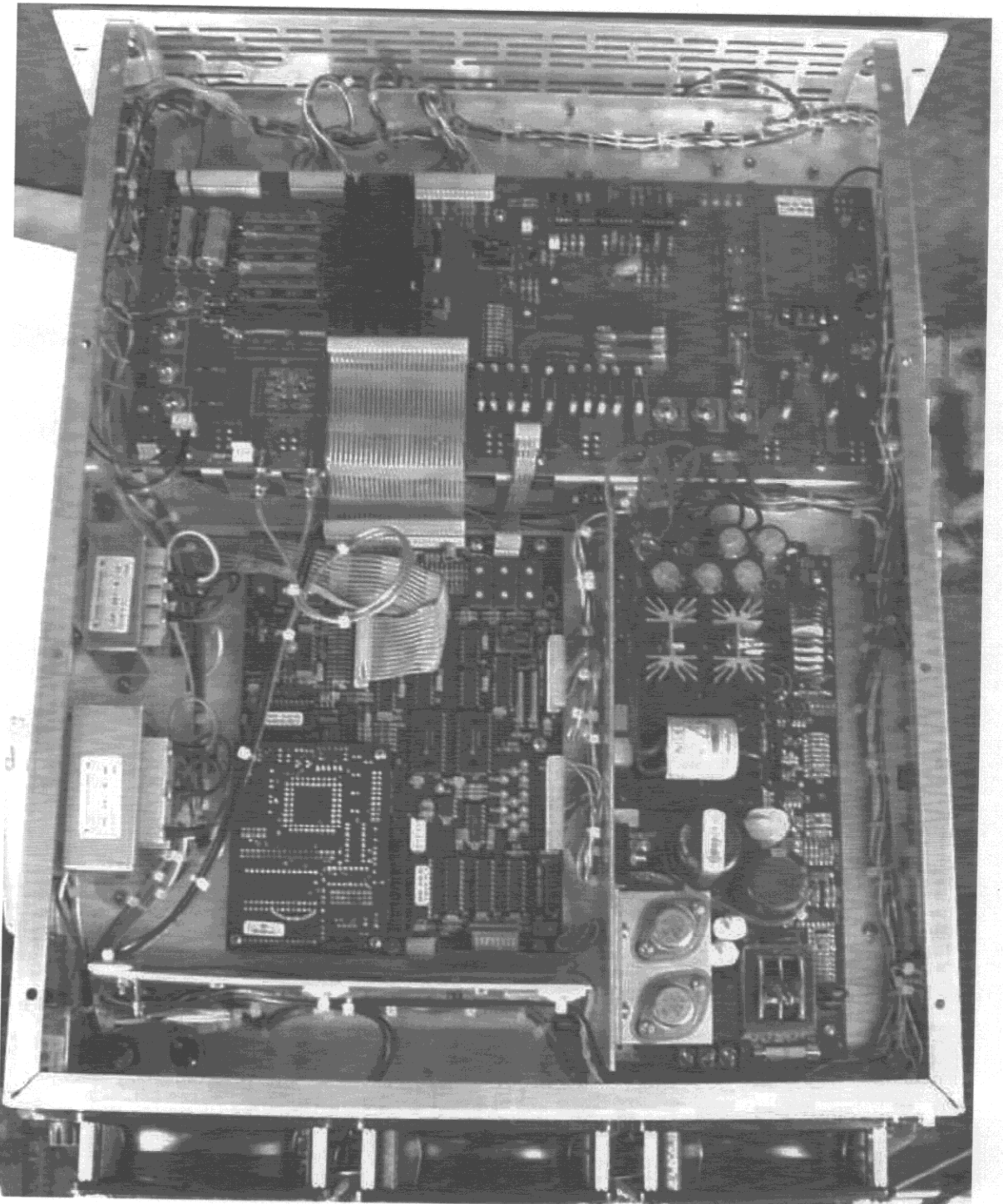
SBM-1000A VHF/UHF TO \mu W UPCONVERTER (DRIVER) BOTTOM VIEW
