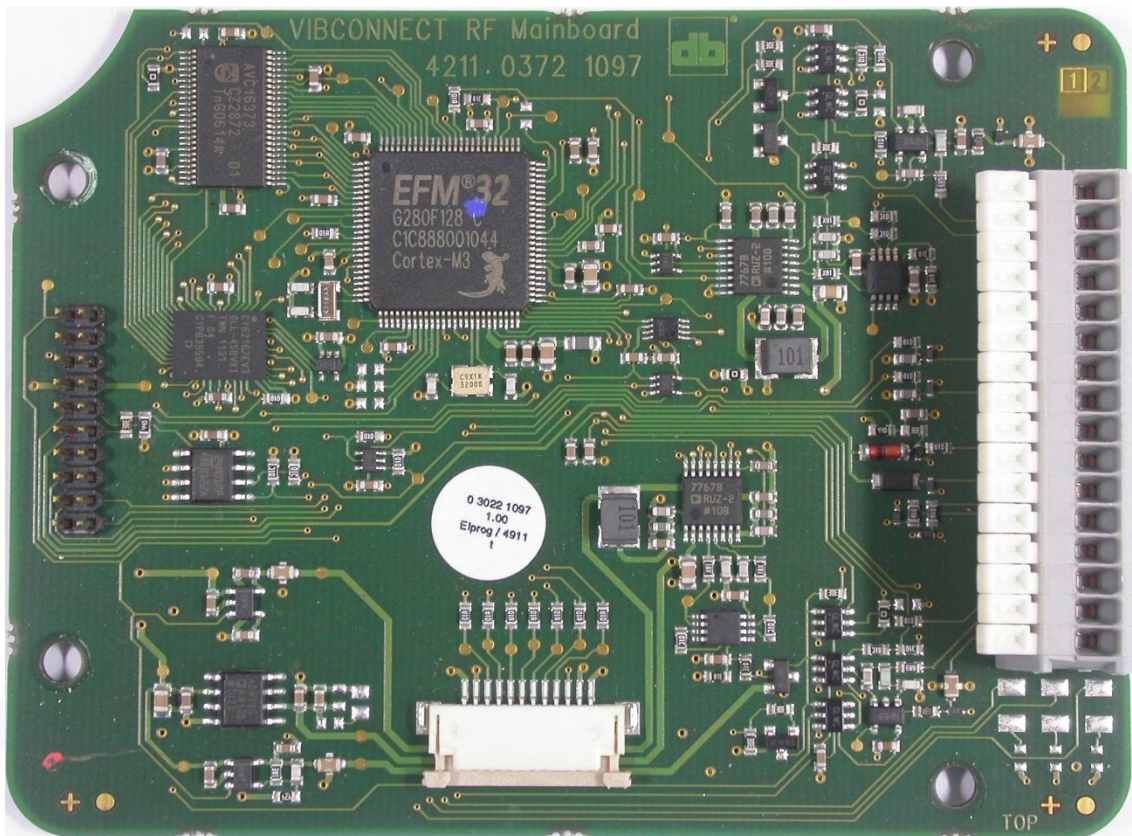
Circuit board 3:
