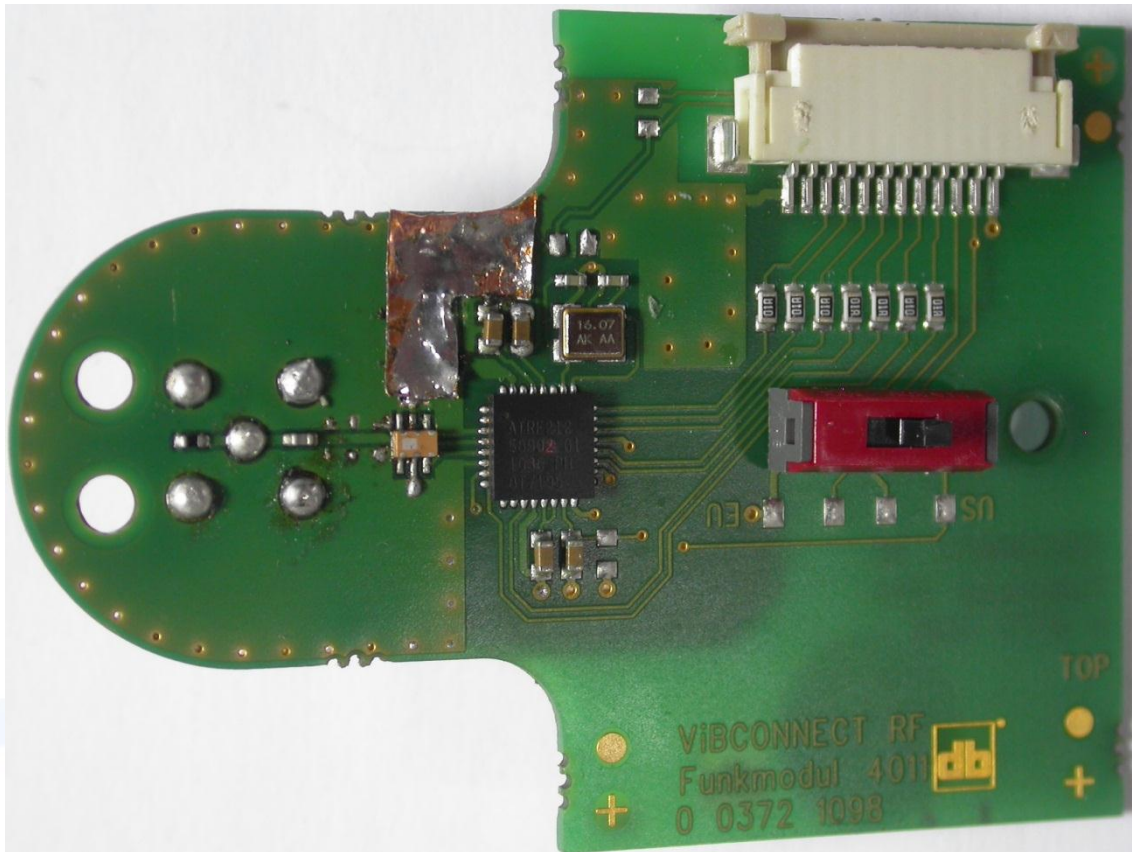
Circuit board 1:
