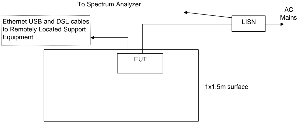
Figure 1. Conducted Emissions Test Setup
