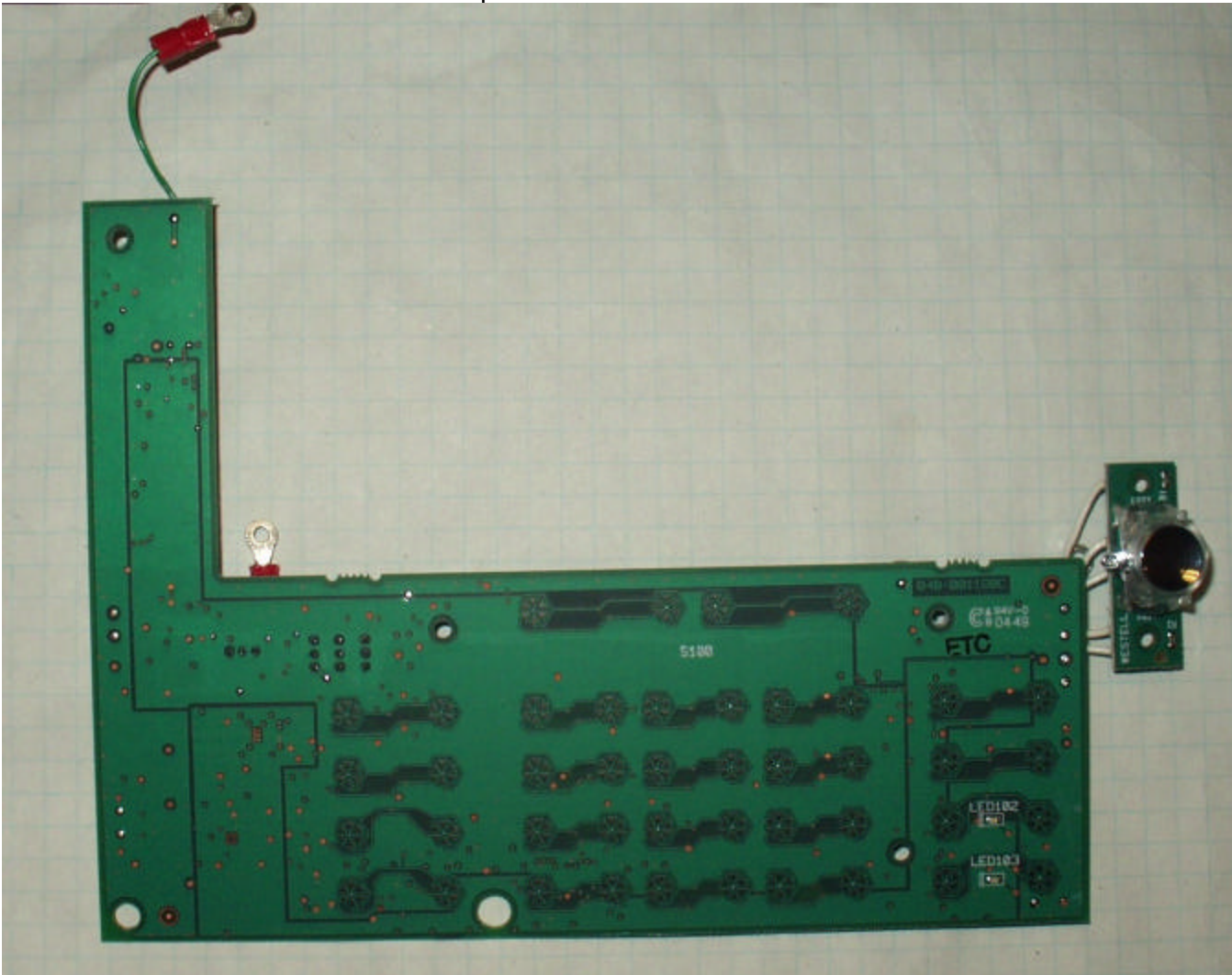
Speaker Board – Foil Side
