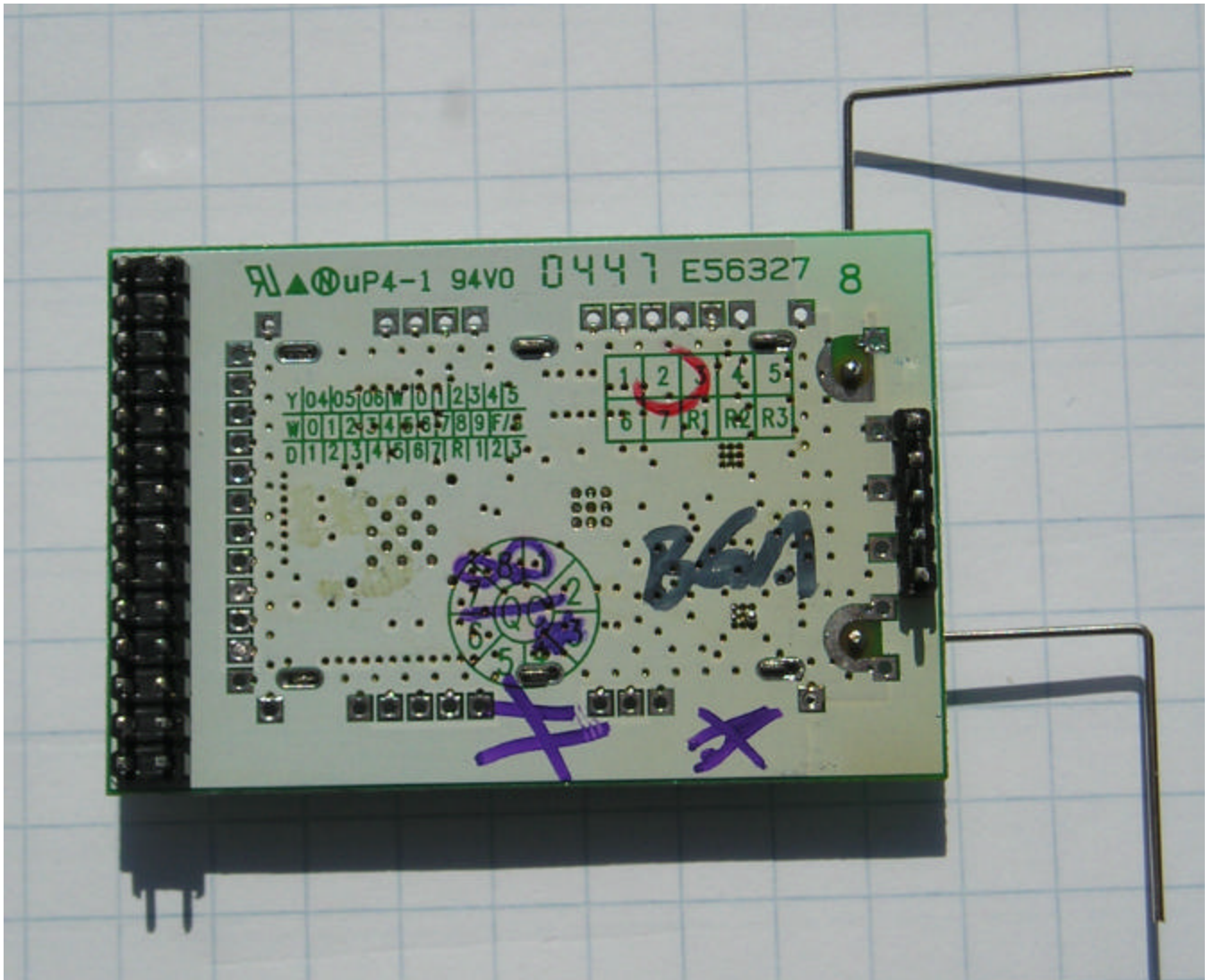
5.8 GHz PCB
