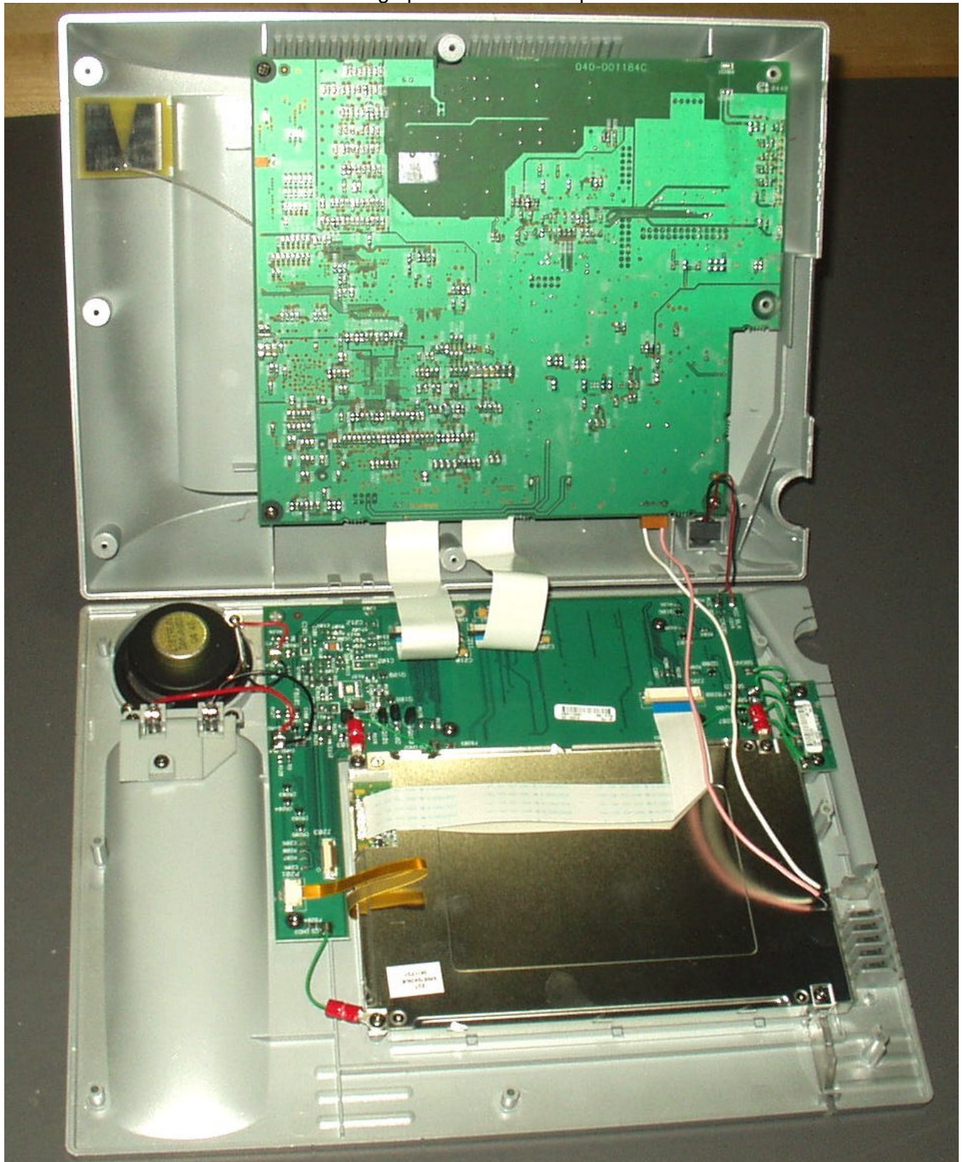
Photograph of EUT - case opened
