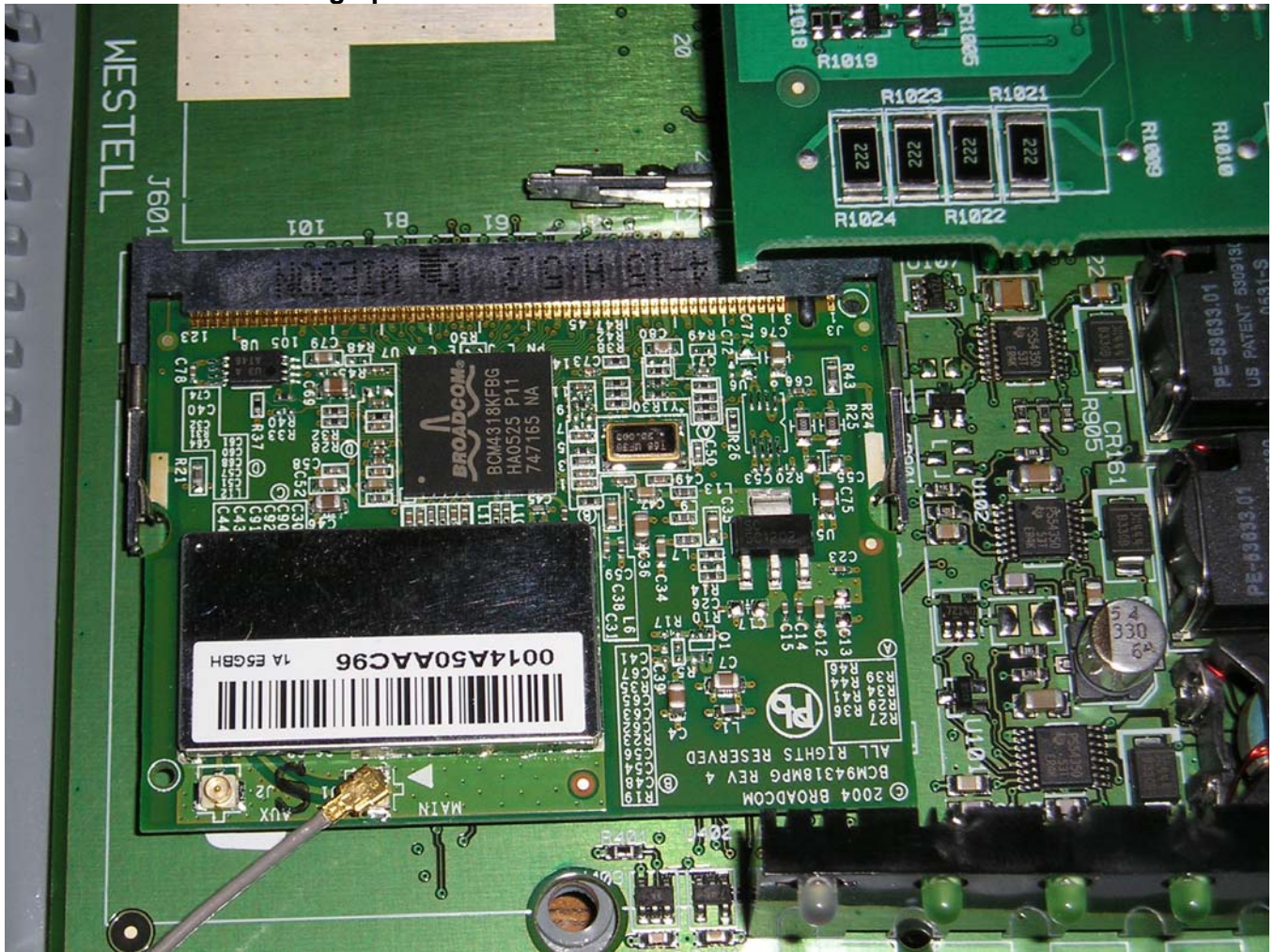
Photograph of Radio Board – As installed on Mother Board
