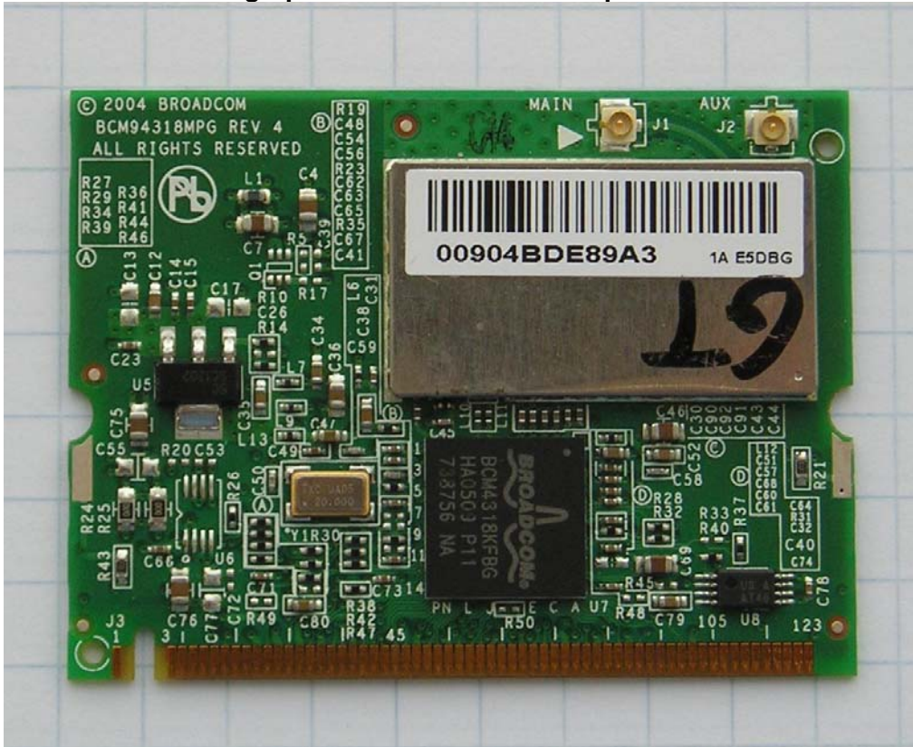
Photograph of Radio Board – Component side
