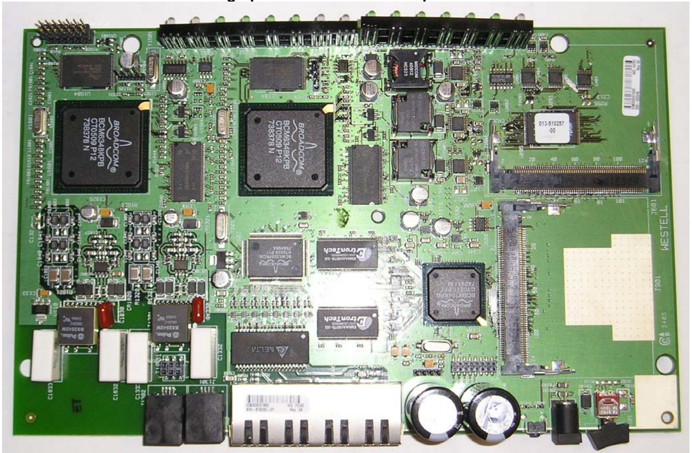
Photograph of Main Board – Component side
