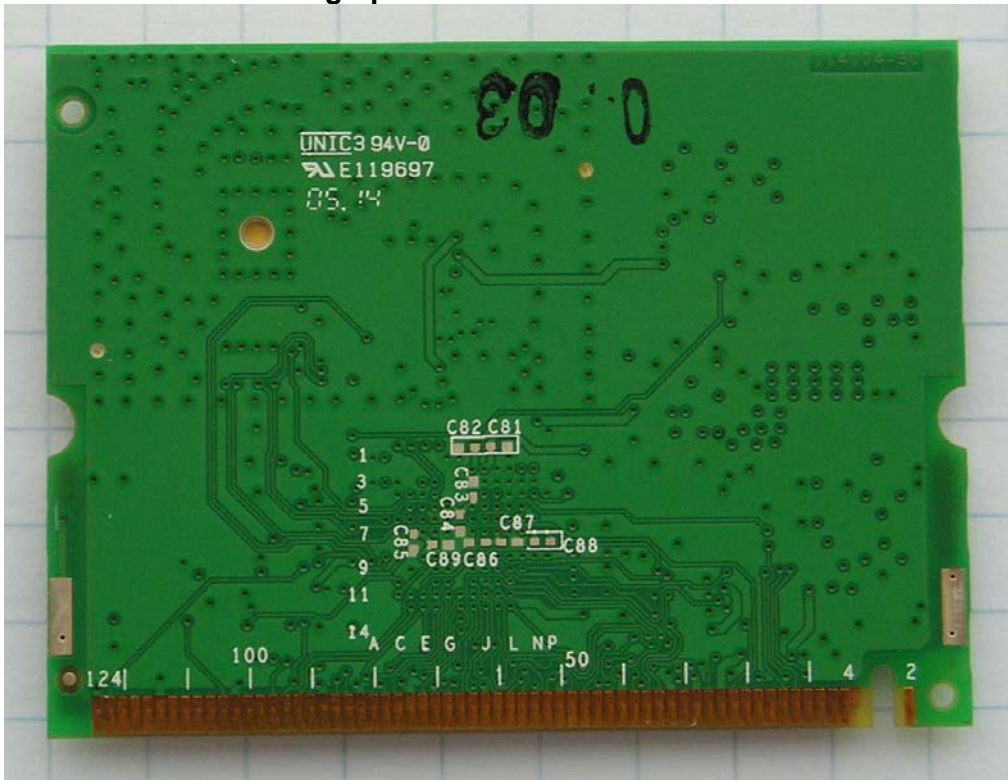
Photograph of Radio Board – Foil side
