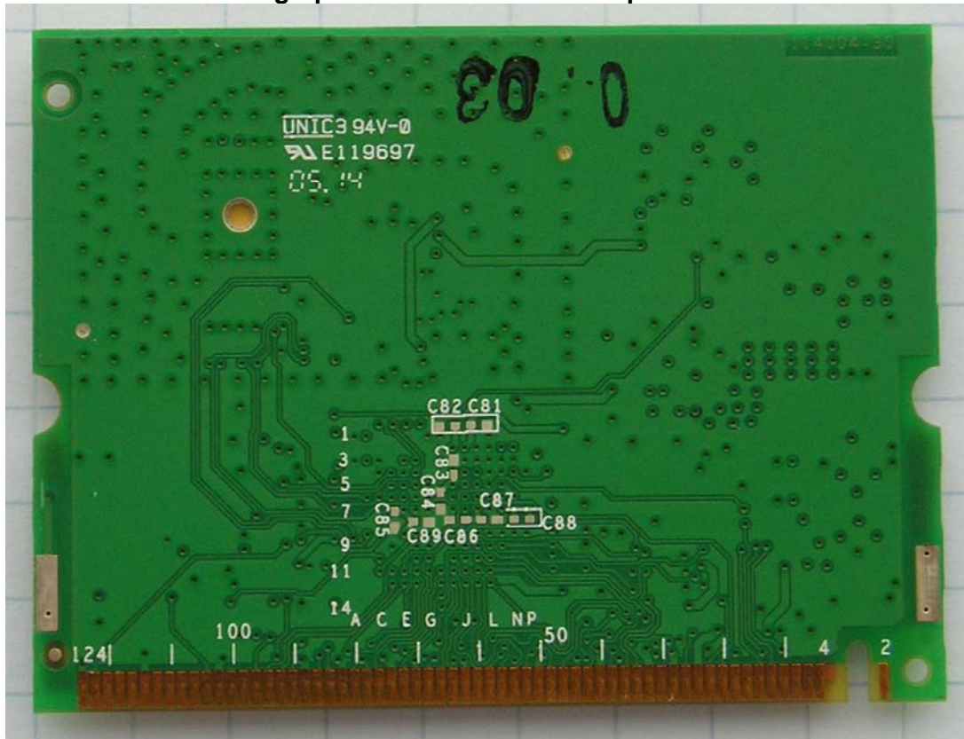
Photograph of Radio Board – Component side
