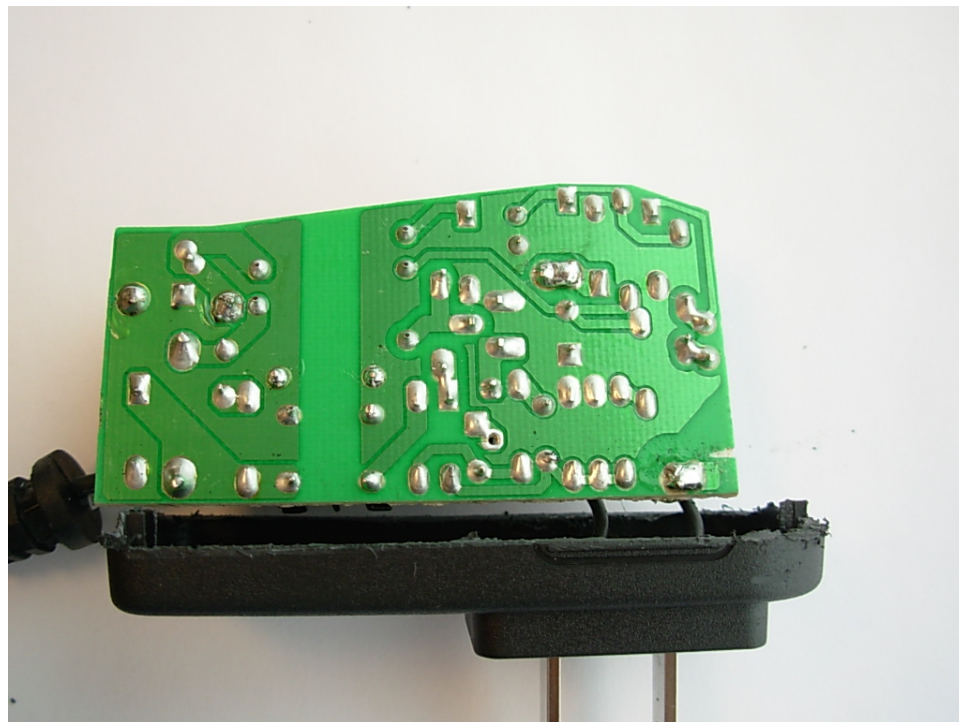
Figure 2. Photograph of Power Supply Board: Foil Side
