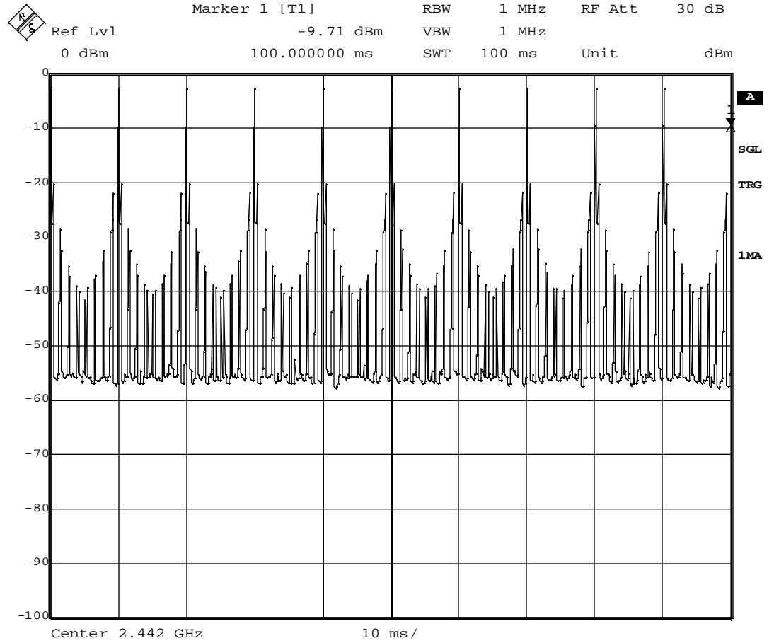
Figure 5: 100 millisecond plot of activity on one channel in page mode
