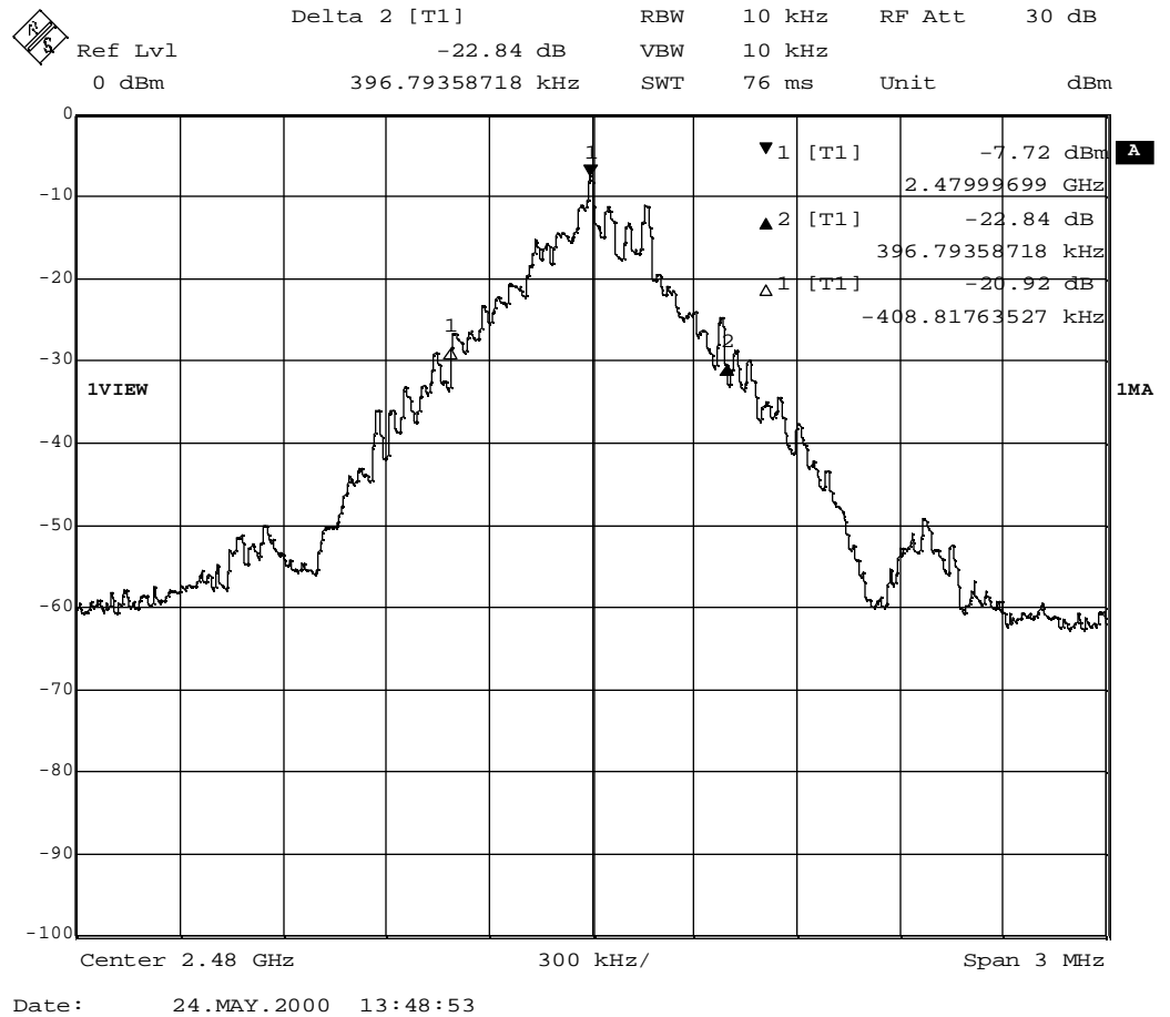
Figure 3: 20 dB bandwidth channel 80 (active mode)
