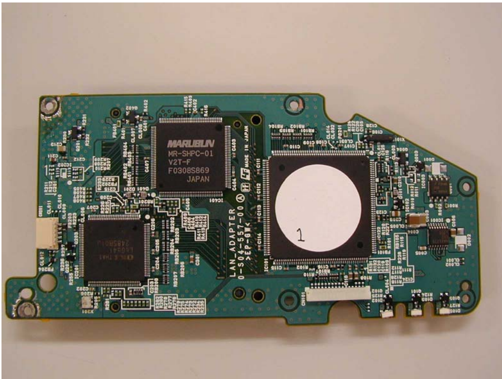
W-LAN Transmitter (Bottom – Cover off)
