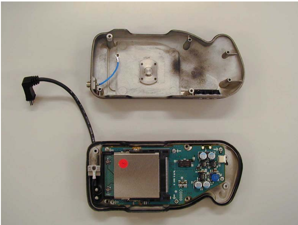
W-LAN Transmitter and Cover
