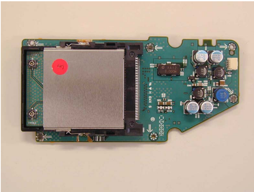
Wireless Transmitter (Top – Cover off)
