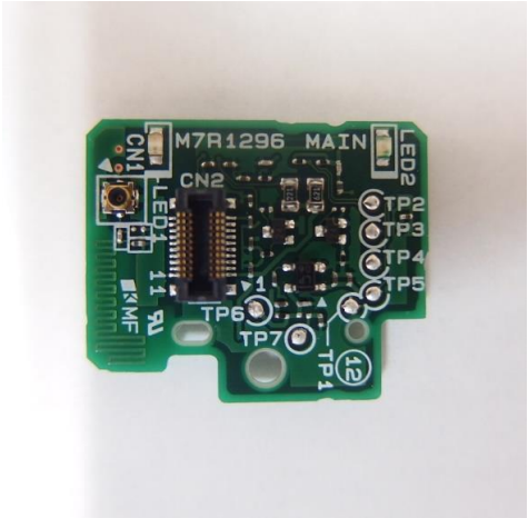
MAIN Back of the board (wireless module)
