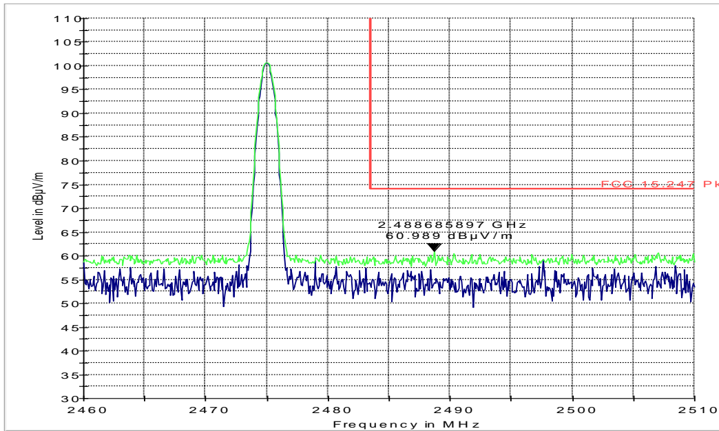
FCC 15.247 HBE Pk 3m
