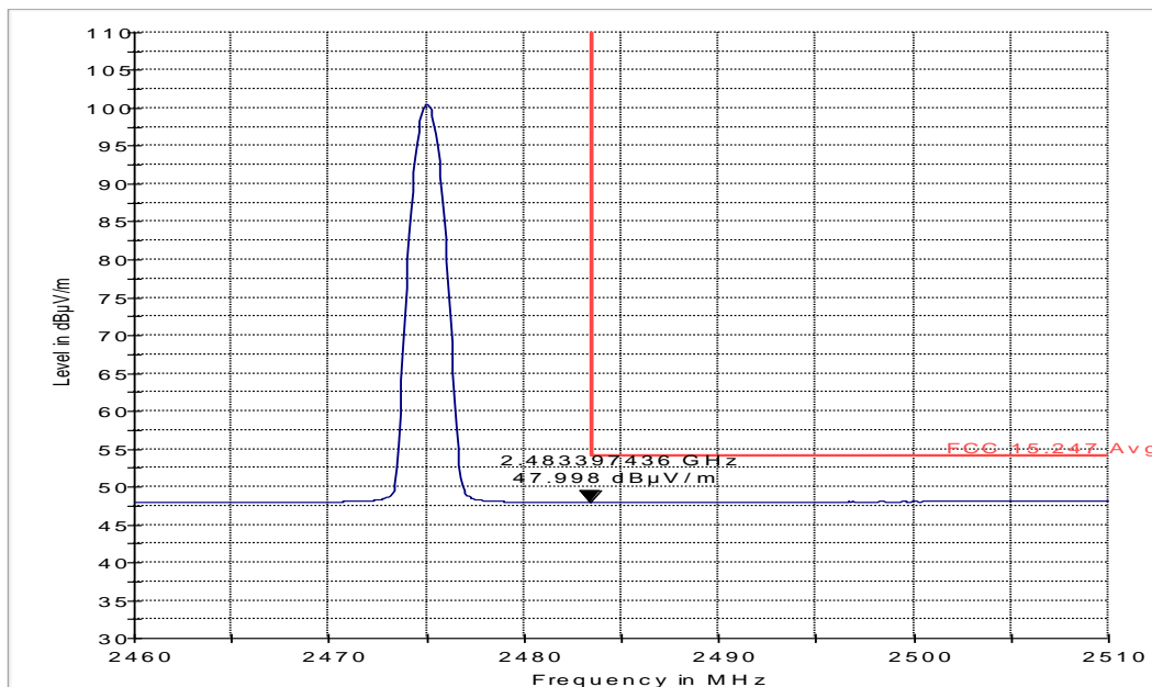
FCC 15.247 HBE Avg 3m
