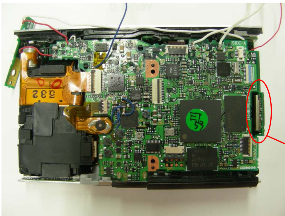
Main PWB
