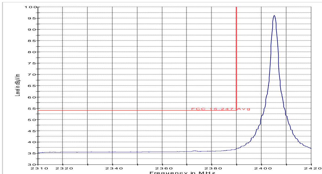
FCC 15.247 LBE Avg 3m
