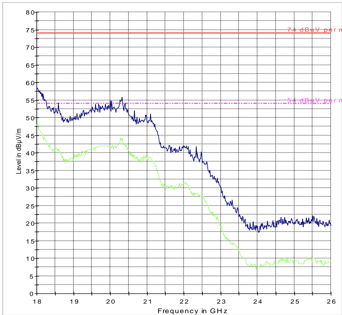
FCC 15 18-26GHz
