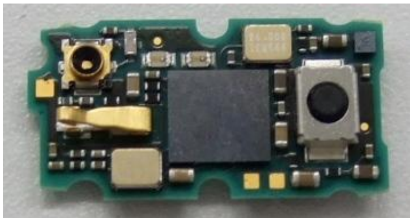
RFBoard (Top)
