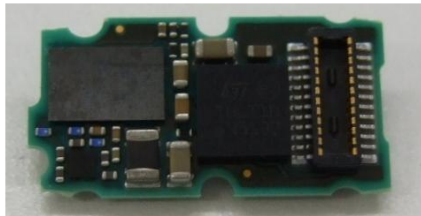
RF Board (Back)
