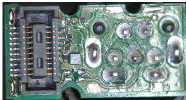
Connector Board(Top)
