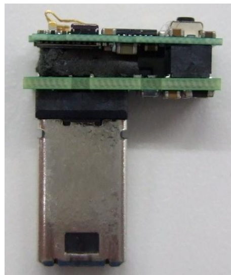
RF Board + Connector Board (Side C)
