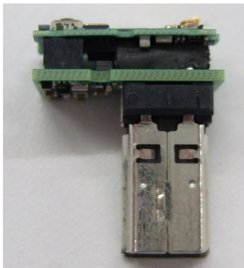
RF Board + Connector Board (Side A)
